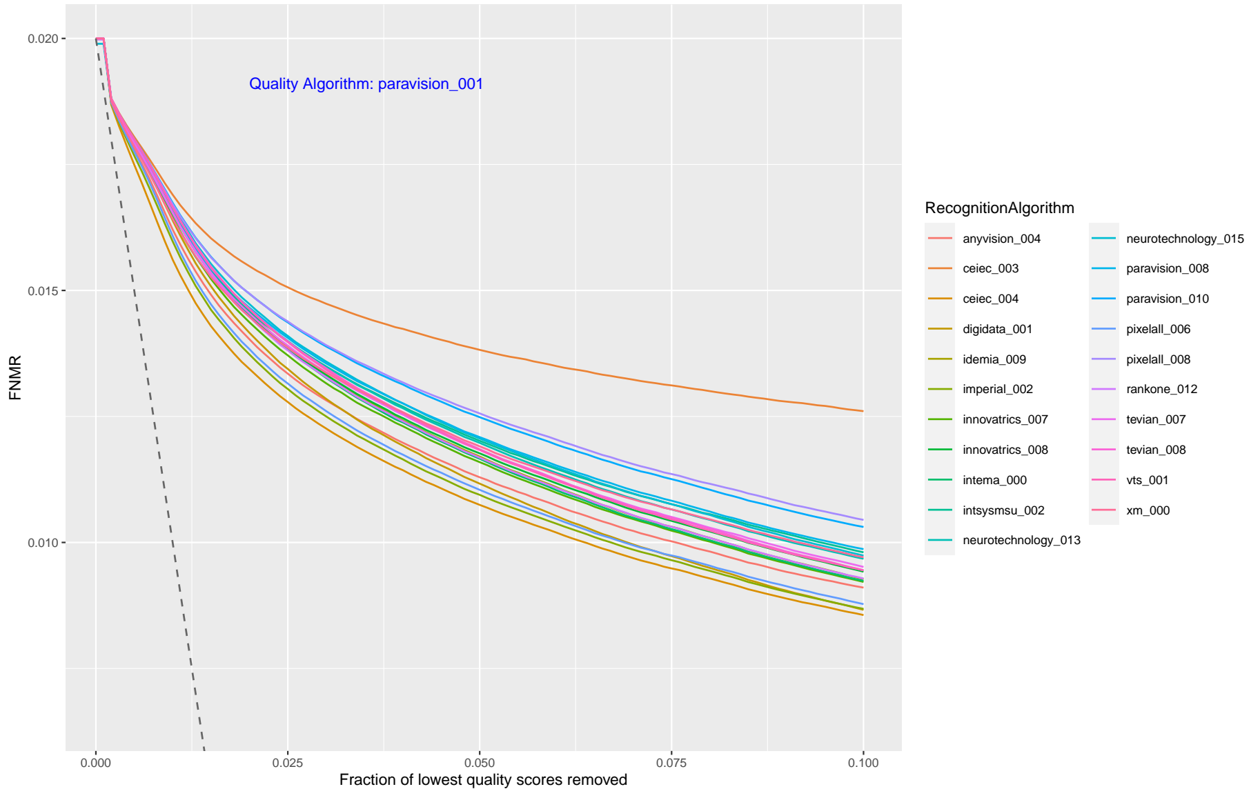
Figure 17: This plot shows FNMR vs. Reject, showing how FNMR reduces when the worst quality data is discarded. Each trace corresponds to a recognition algorithm, and each page corresponds to one quality assessment algorithm. The quality score is from the verification (webcam) border crossing image. A perfect quality algorithm would predict which images are implicated in false non-matches. This is shown by the grey dotted line ( \max((FNMR - x), 0) ). The closer the quality algorithm line is to the perfect line, the better the quality prediction performance is relative to recognition outcomes.
