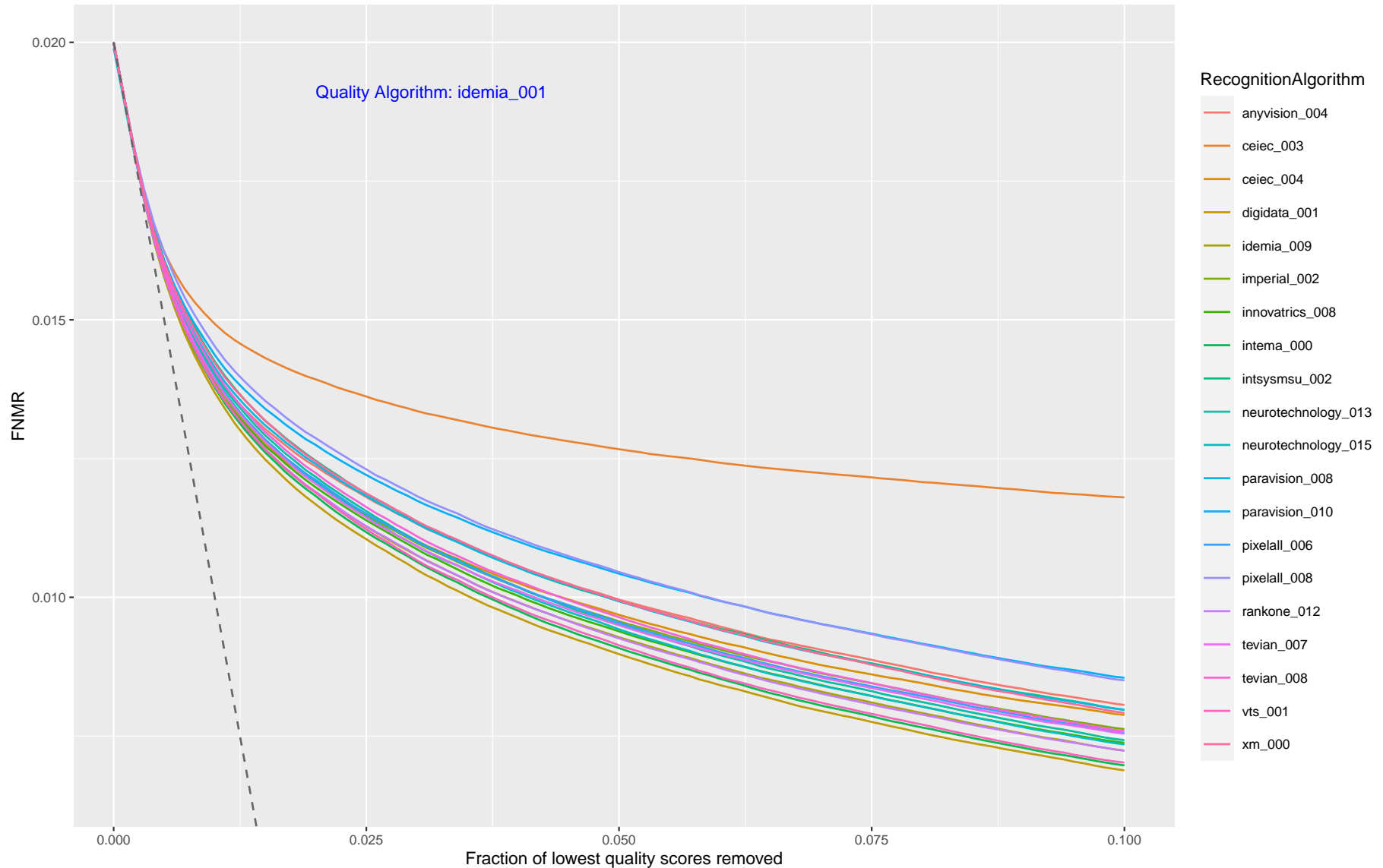
Figure 13: This plot shows FNMR vs. Reject, showing how FNMR reduces when the worst quality data is discarded. Each trace corresponds to a recognition algorithm, and each page corresponds to one quality assessment algorithm. The quality score is from the verification (webcam) border crossing image. A perfect quality algorithm would predict which images are implicated in false non-matches. This is shown by the grey dotted line ( \max((FNMR - x), 0) ). The closer the quality algorithm line is to the perfect line, the better the quality prediction performance is relative to recognition outcomes.
