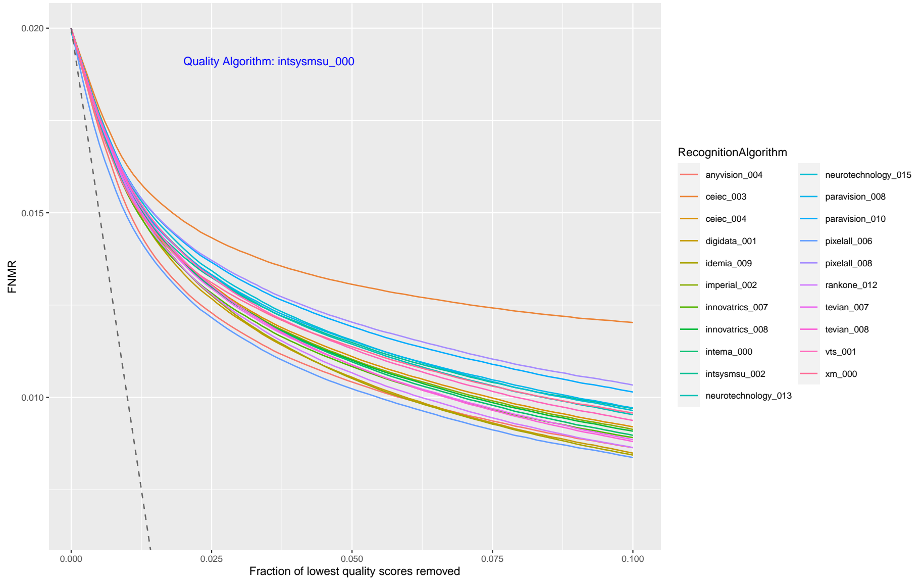
Figure 15: This plot shows FNMR vs. Reject, showing how FNMR reduces when the worst quality data is discarded. Each trace corresponds to a recognition algorithm, and each page corresponds to one quality assessment algorithm. The quality score is from the verification (webcam) border crossing image. A perfect quality algorithm would predict which images are implicated in false non-matches. This is shown by the grey dotted line ( \max((FNMR - x), 0) ). The closer the quality algorithm line is to the perfect line, the better the quality prediction performance is relative to recognition outcomes.
