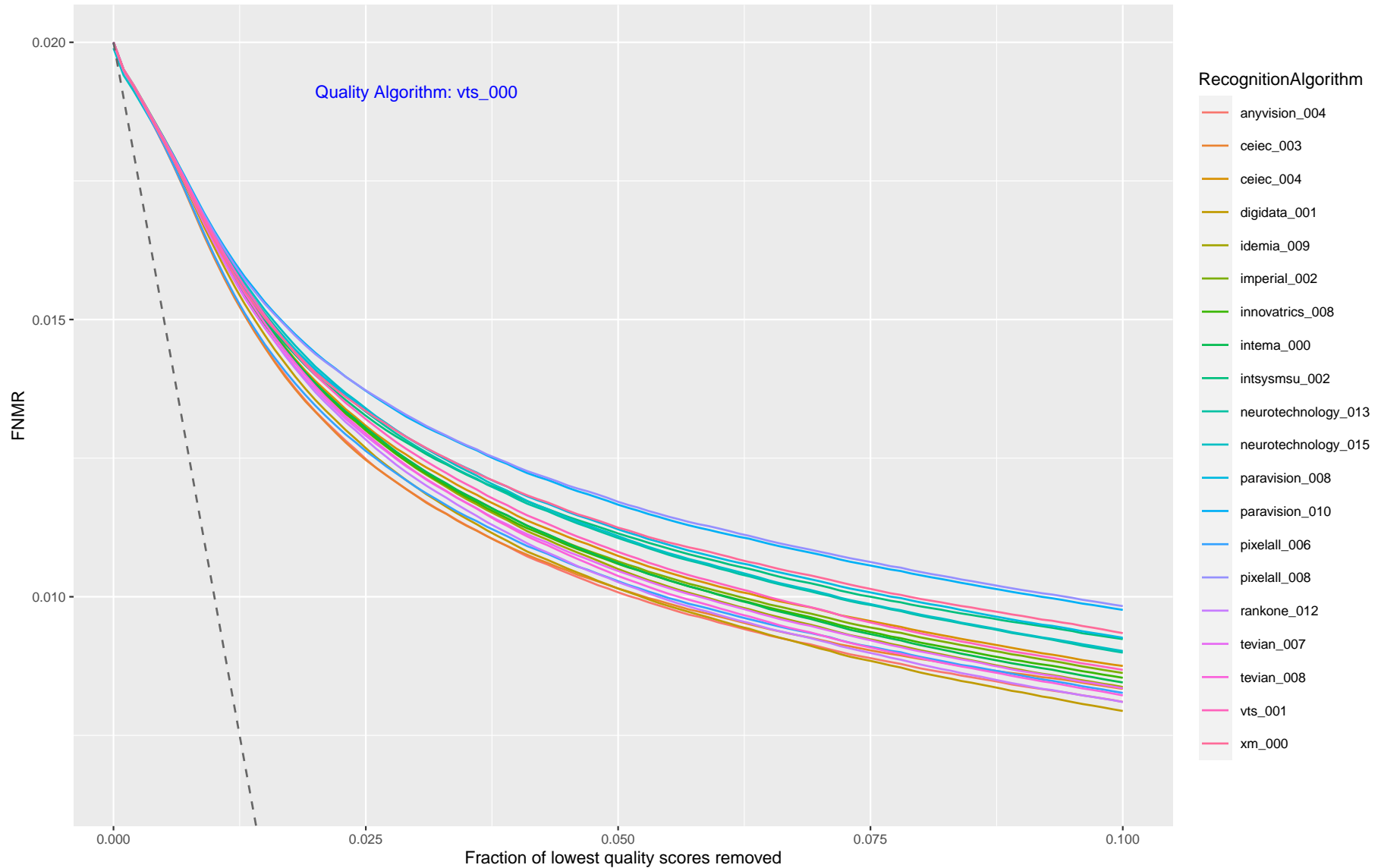
Figure 27: This plot shows FNMR vs. Reject, showing how FNMR reduces when the worst quality data is discarded. Each trace corresponds to a recognition algorithm, and each page corresponds to one quality assessment algorithm. The quality score is from the verification (webcam) border crossing image. A perfect quality algorithm would predict which images are implicated in false non-matches. This is shown by the grey dotted line ( \max((FNMR - x), 0) ). The closer the quality algorithm line is to the perfect line, the better the quality prediction performance is relative to recognition outcomes.
