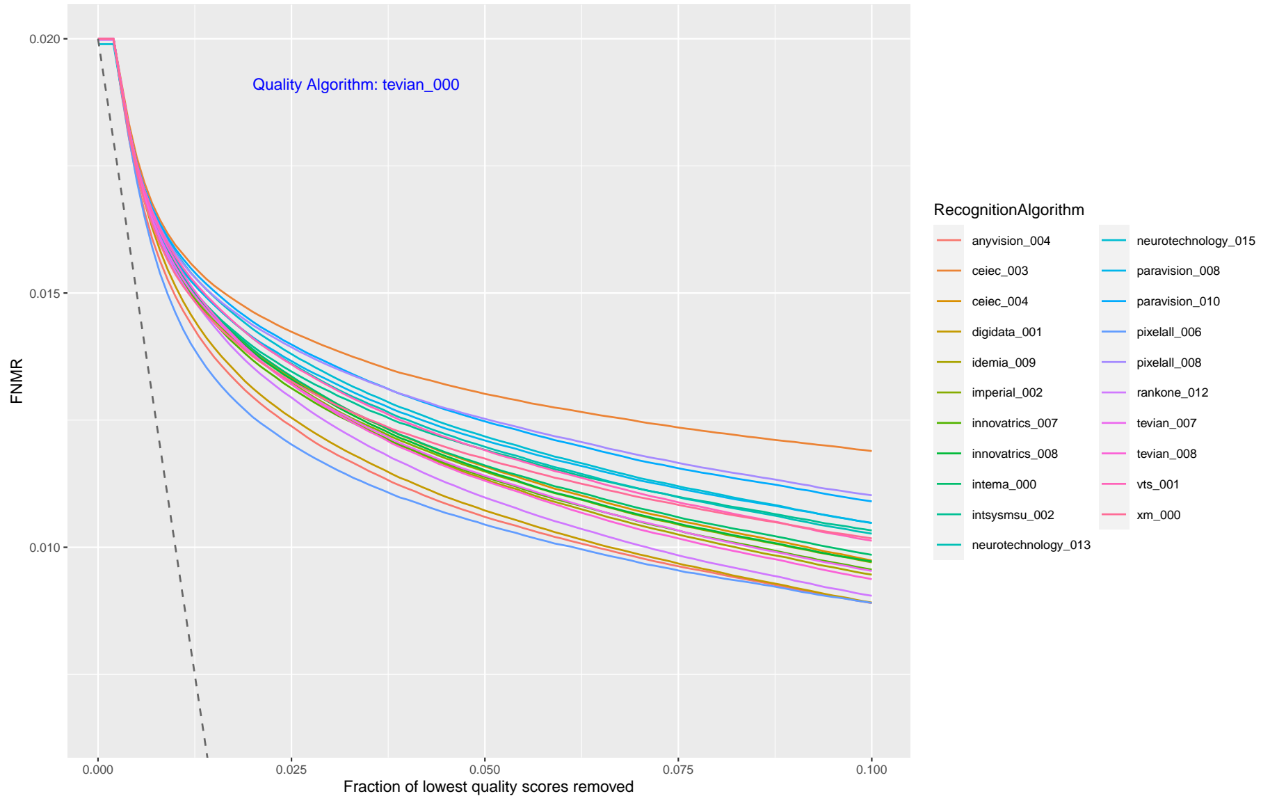
Figure 24: This plot shows FNMR vs. Reject, showing how FNMR reduces when the worst quality data is discarded. Each trace corresponds to a recognition algorithm, and each page corresponds to one quality assessment algorithm. The quality score is from the verification (webcam) border crossing image. A perfect quality algorithm would predict which images are implicated in false non-matches. This is shown by the grey dotted line ( \max((FNMR - x), 0) ). The closer the quality algorithm line is to the perfect line, the better the quality prediction performance is relative to recognition outcomes.
