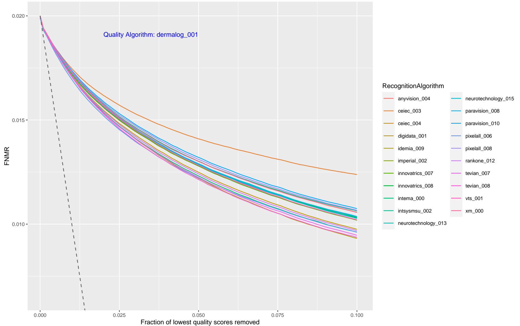
Figure 11: This plot shows FNMR vs. Reject, showing how FNMR reduces when the worst quality data is discarded. Each trace corresponds to a recognition algorithm, and each page corresponds to one quality assessment algorithm. The quality score is from the verification (webcam) border crossing image. A perfect quality algorithm would predict which images are implicated in false non-matches. This is shown by the grey dotted line ( \max((FNMR - x), 0) ). The closer the quality algorithm line is to the perfect line, the better the quality prediction performance is relative to recognition outcomes.
