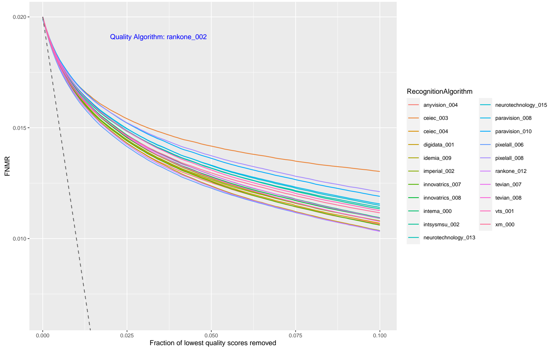
Figure 21: This plot shows FNMR vs. Reject, showing how FNMR reduces when the worst quality data is discarded. Each trace corresponds to a recognition algorithm, and each page corresponds to one quality assessment algorithm. The quality score is from the verification (webcam) border crossing image. A perfect quality algorithm would predict which images are implicated in false non-matches. This is shown by the grey dotted line ( \max((FNMR - x), 0) ). The closer the quality algorithm line is to the perfect line, the better the quality prediction performance is relative to recognition outcomes.
