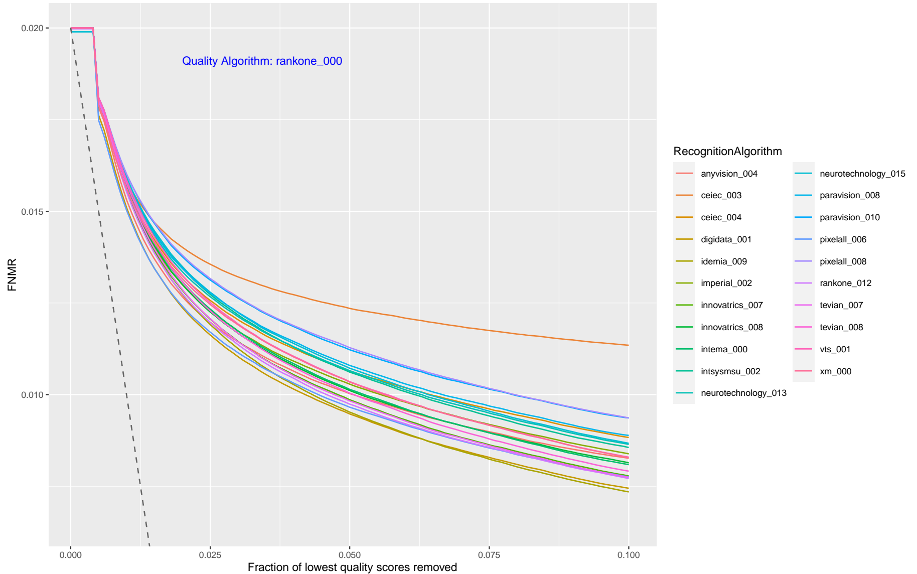
Figure 19: This plot shows FNMR vs. Reject, showing how FNMR reduces when the worst quality data is discarded. Each trace corresponds to a recognition algorithm, and each page corresponds to one quality assessment algorithm. The quality score is from the verification (webcam) border crossing image. A perfect quality algorithm would predict which images are implicated in false non-matches. This is shown by the grey dotted line ( \max((FNMR - x), 0) ). The closer the quality algorithm line is to the perfect line, the better the quality prediction performance is relative to recognition outcomes.
