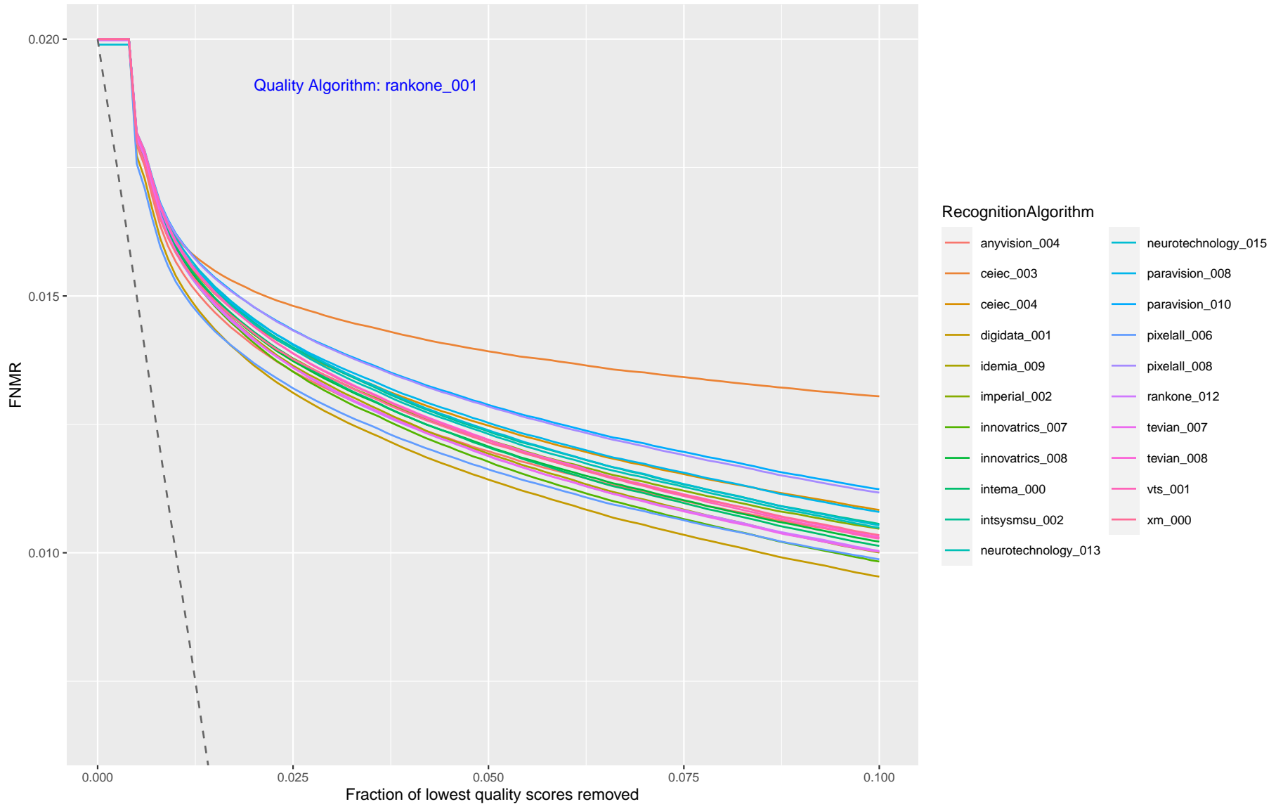
Figure 20: This plot shows FNMR vs. Reject, showing how FNMR reduces when the worst quality data is discarded. Each trace corresponds to a recognition algorithm, and each page corresponds to one quality assessment algorithm. The quality score is from the verification (webcam) border crossing image. A perfect quality algorithm would predict which images are implicated in false non-matches. This is shown by the grey dotted line ( \max((FNMR - x), 0) ). The closer the quality algorithm line is to the perfect line, the better the quality prediction performance is relative to recognition outcomes.
