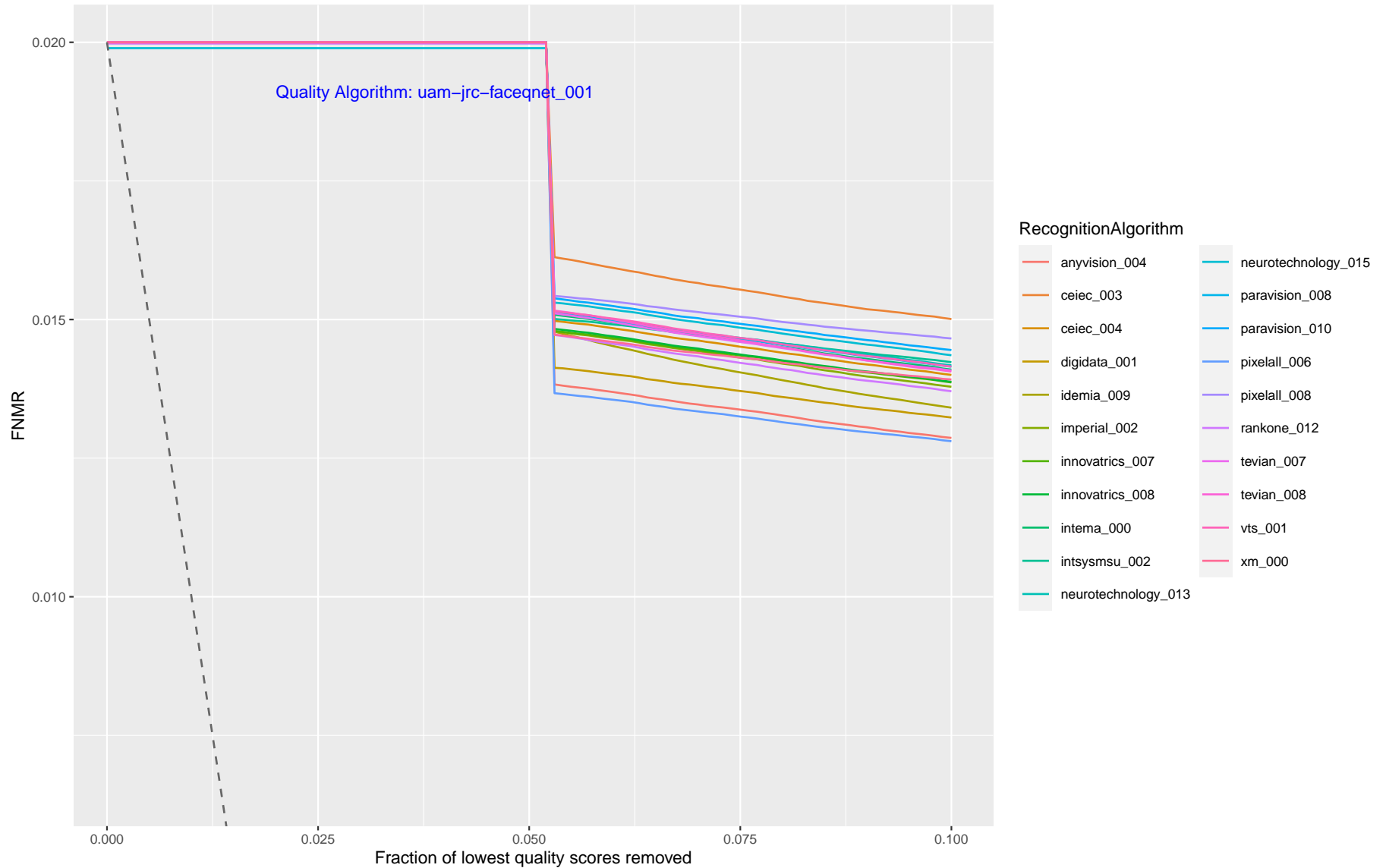
Figure 26: This plot shows FNMR vs. Reject, showing how FNMR reduces when the worst quality data is discarded. Each trace corresponds to a recognition algorithm, and each page corresponds to one quality assessment algorithm. The quality score is from the verification (webcam) border crossing image. A perfect quality algorithm would predict which images are implicated in false non-matches. This is shown by the grey dotted line ( \max((FNMR - x), 0) ). The closer the quality algorithm line is to the perfect line, the better the quality prediction performance is relative to recognition outcomes.
