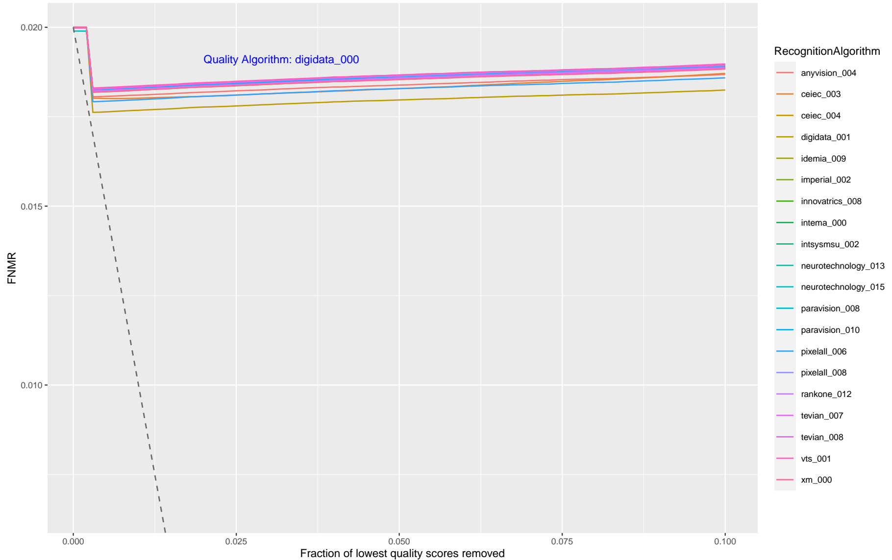
Figure 12: This plot shows FNMR vs. Reject, showing how FNMR reduces when the worst quality data is discarded. Each trace corresponds to a recognition algorithm, and each page corresponds to one quality assessment algorithm. The quality score is from the verification (webcam) border crossing image. A perfect quality algorithm would predict which images are implicated in false non-matches. This is shown by the grey dotted line ( \max((FNMR - x), 0) ). The closer the quality algorithm line is to the perfect line, the better the quality prediction performance is relative to recognition outcomes.
