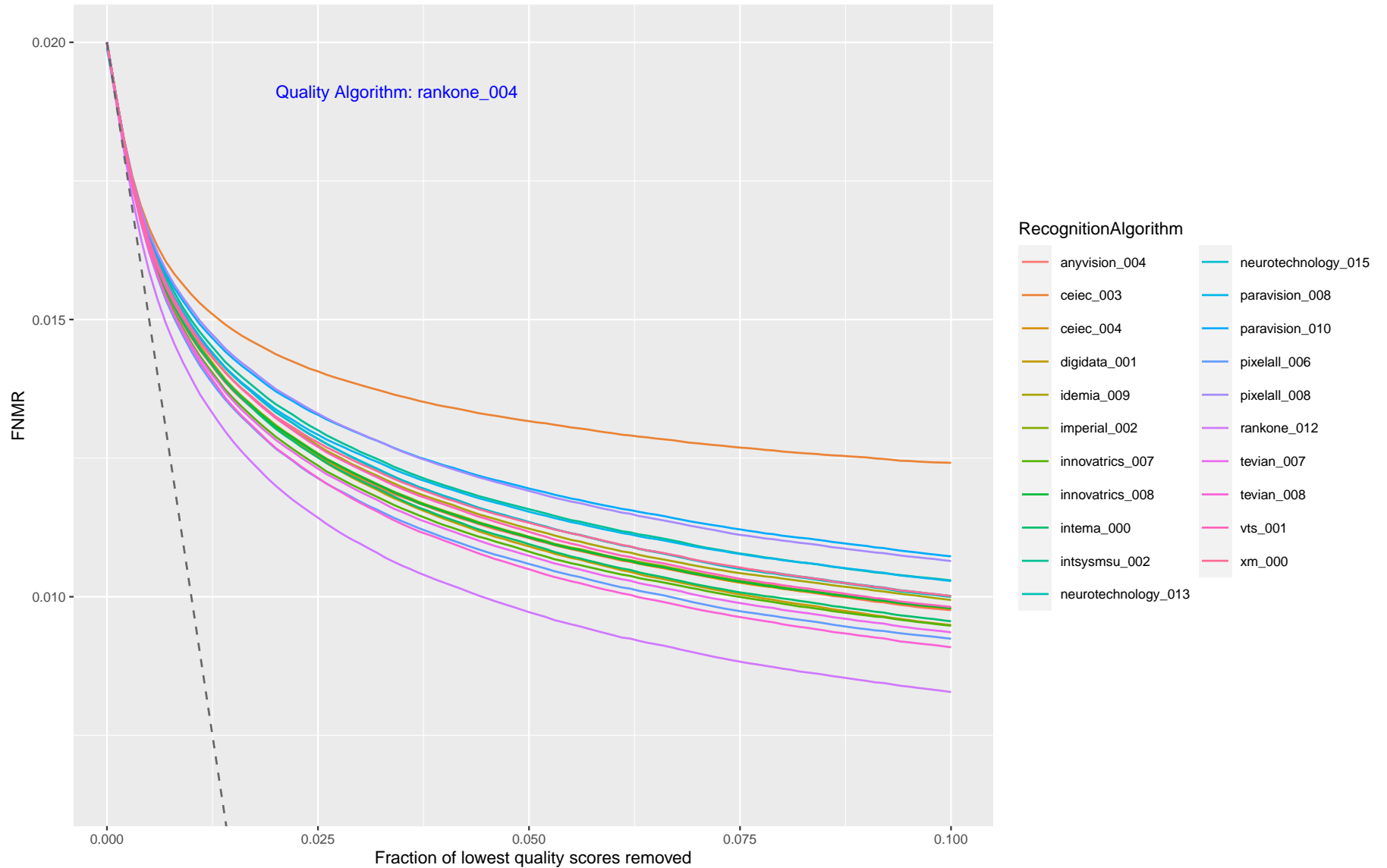
Figure 23: This plot shows FNMR vs. Reject, showing how FNMR reduces when the worst quality data is discarded. Each trace corresponds to a recognition algorithm, and each page corresponds to one quality assessment algorithm. The quality score is from the verification (webcam) border crossing image. A perfect quality algorithm would predict which images are implicated in false non-matches. This is shown by the grey dotted line ( \max((FNMR - x), 0) ). The closer the quality algorithm line is to the perfect line, the better the quality prediction performance is relative to recognition outcomes.
