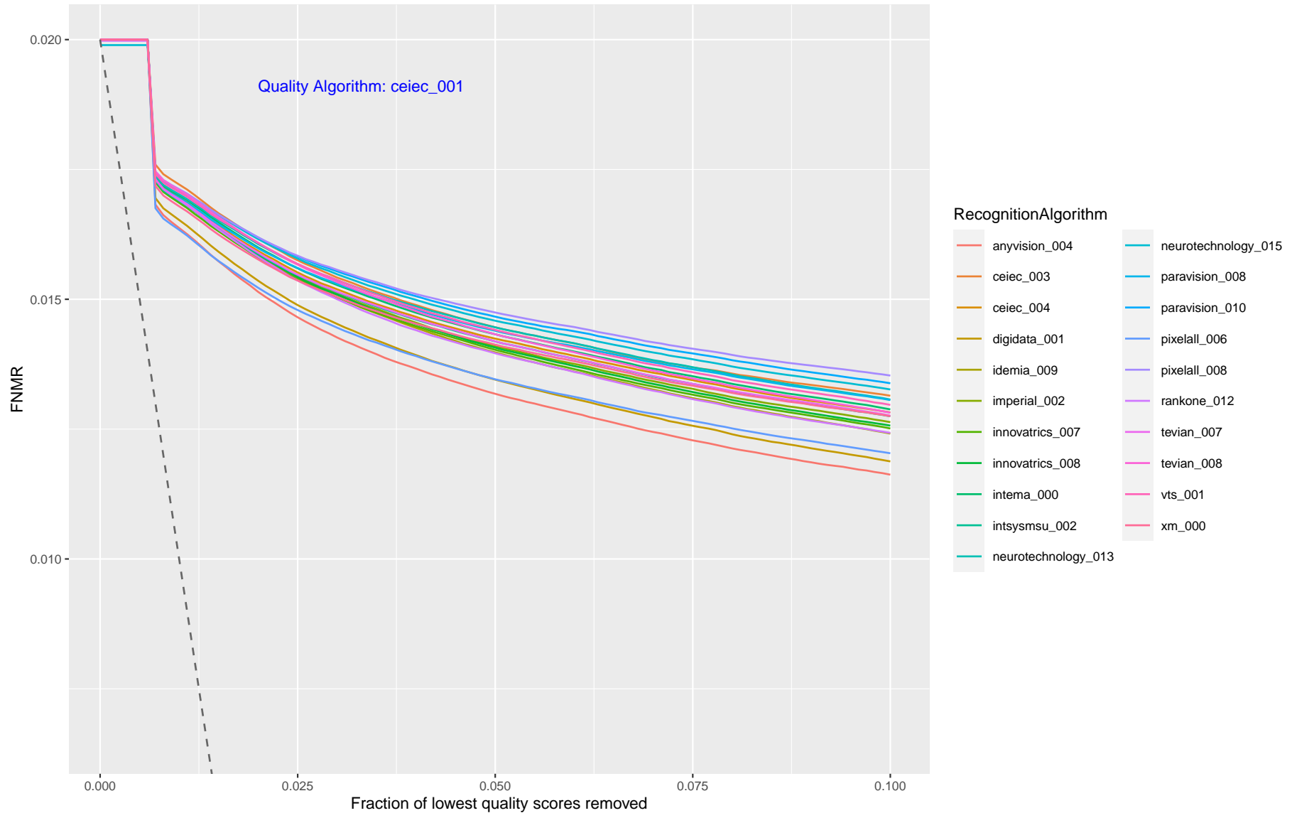
Figure 10: This plot shows FNMR vs. Reject, showing how FNMR reduces when the worst quality data is discarded. Each trace corresponds to a recognition algorithm, and each page corresponds to one quality assessment algorithm. The quality score is from the verification (webcam) border crossing image. A perfect quality algorithm would predict which images are implicated in false non-matches. This is shown by the grey dotted line ( \max((FNMR - x), 0) ). The closer the quality algorithm line is to the perfect line, the better the quality prediction performance is relative to recognition outcomes.
