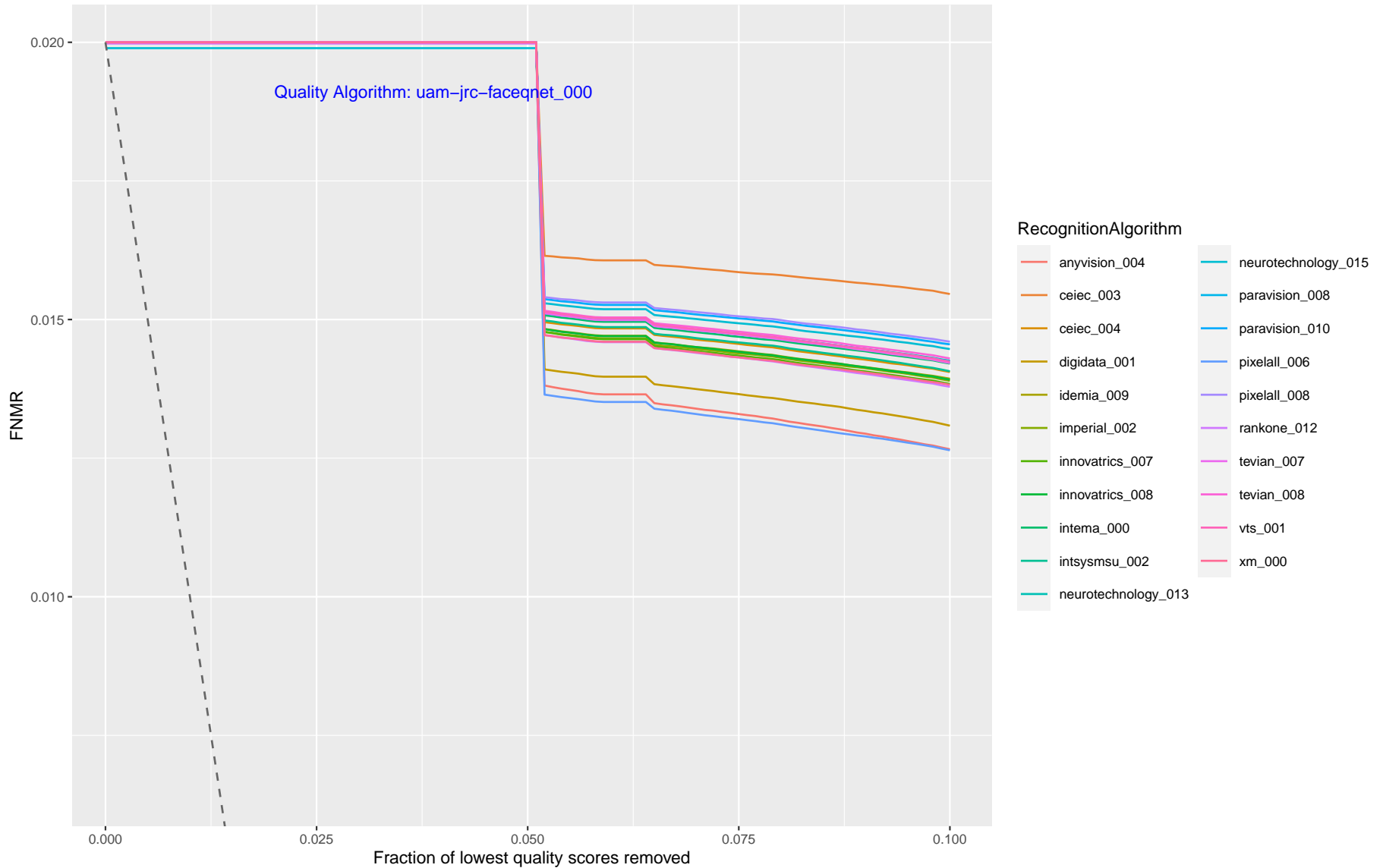
Figure 25: This plot shows FNMR vs. Reject, showing how FNMR reduces when the worst quality data is discarded. Each trace corresponds to a recognition algorithm, and each page corresponds to one quality assessment algorithm. The quality score is from the verification (webcam) border crossing image. A perfect quality algorithm would predict which images are implicated in false non-matches. This is shown by the grey dotted line ( \max((FNMR - x), 0) ). The closer the quality algorithm line is to the perfect line, the better the quality prediction performance is relative to recognition outcomes.
