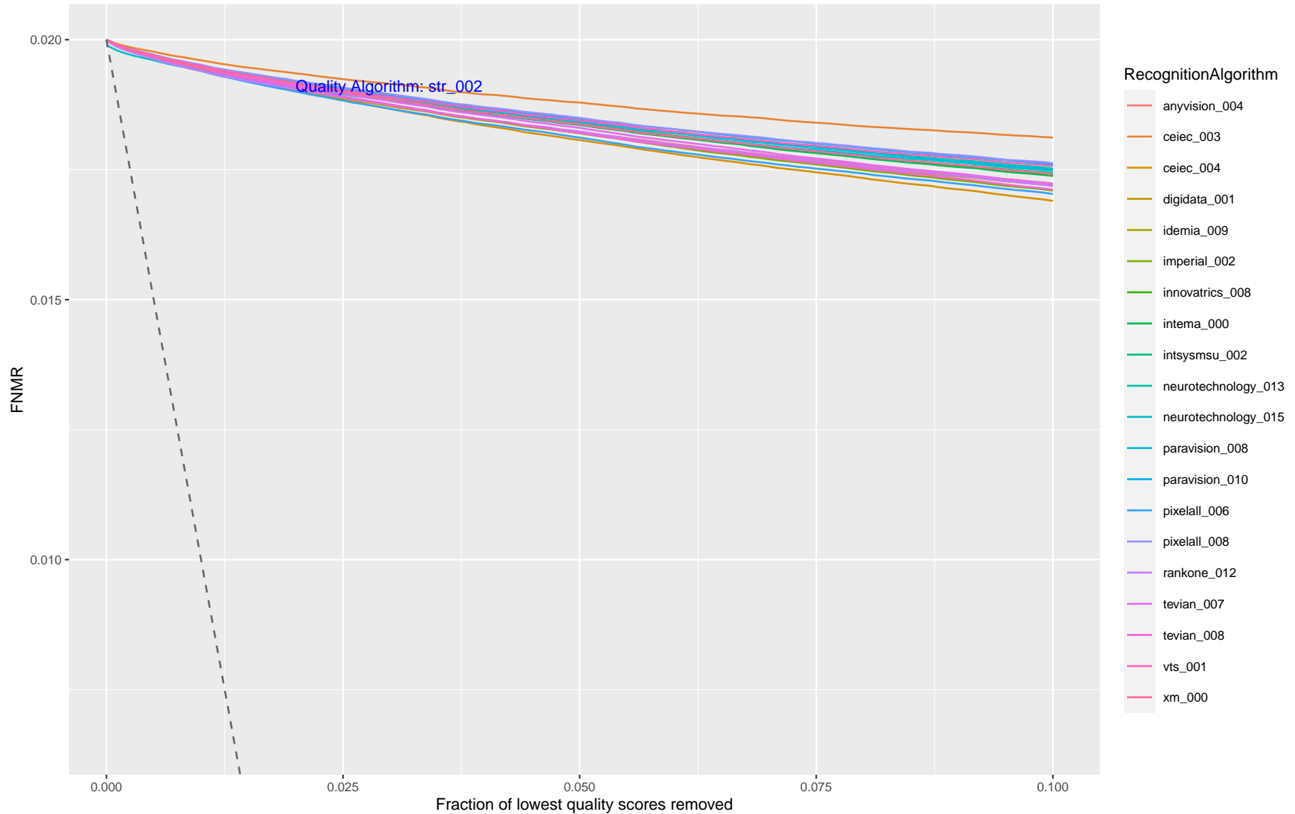
Figure 29: This plot shows FNMR vs. Reject, showing how FNMR reduces when the worst quality data is discarded. Each trace corresponds to a recognition algorithm, and each page corresponds to one quality assessment algorithm. The quality score is from the verification (webcam) border crossing image. A perfect quality algorithm would predict which images are implicated in false non-matches. This is shown by the grey dotted line ( \max((FNMR - x), 0) ). The closer the quality algorithm line is to the perfect line, the better the quality prediction performance is relative to recognition outcomes.
