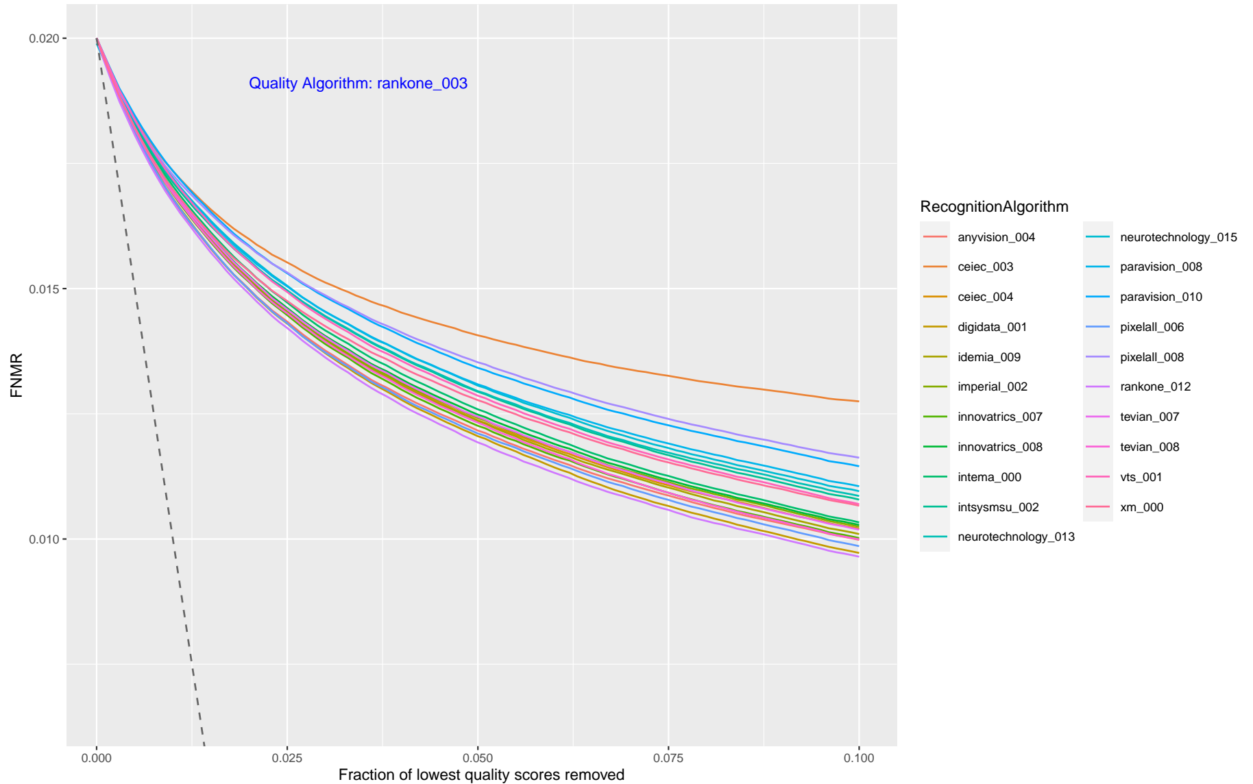
Figure 22: This plot shows FNMR vs. Reject, showing how FNMR reduces when the worst quality data is discarded. Each trace corresponds to a recognition algorithm, and each page corresponds to one quality assessment algorithm. The quality score is from the verification (webcam) border crossing image. A perfect quality algorithm would predict which images are implicated in false non-matches. This is shown by the grey dotted line ( \max((FNMR - x), 0) ). The closer the quality algorithm line is to the perfect line, the better the quality prediction performance is relative to recognition outcomes.
