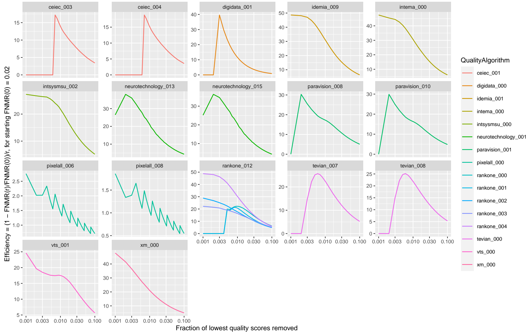
Figure 30: This plot is a simple modification of the prior figure. It shows efficiency vs. rejection, where the y-axis shows FNMR divided by the perfect FNMR i.e. how efficient the quality reject mechanism is. A value of 1 indicates perfect rejection of the low quality images. Each panel corresponds to a recognition algorithm, and the lines within each panel correspond to quality assessment algorithms. The quality score is from the verification (webcam) image.
