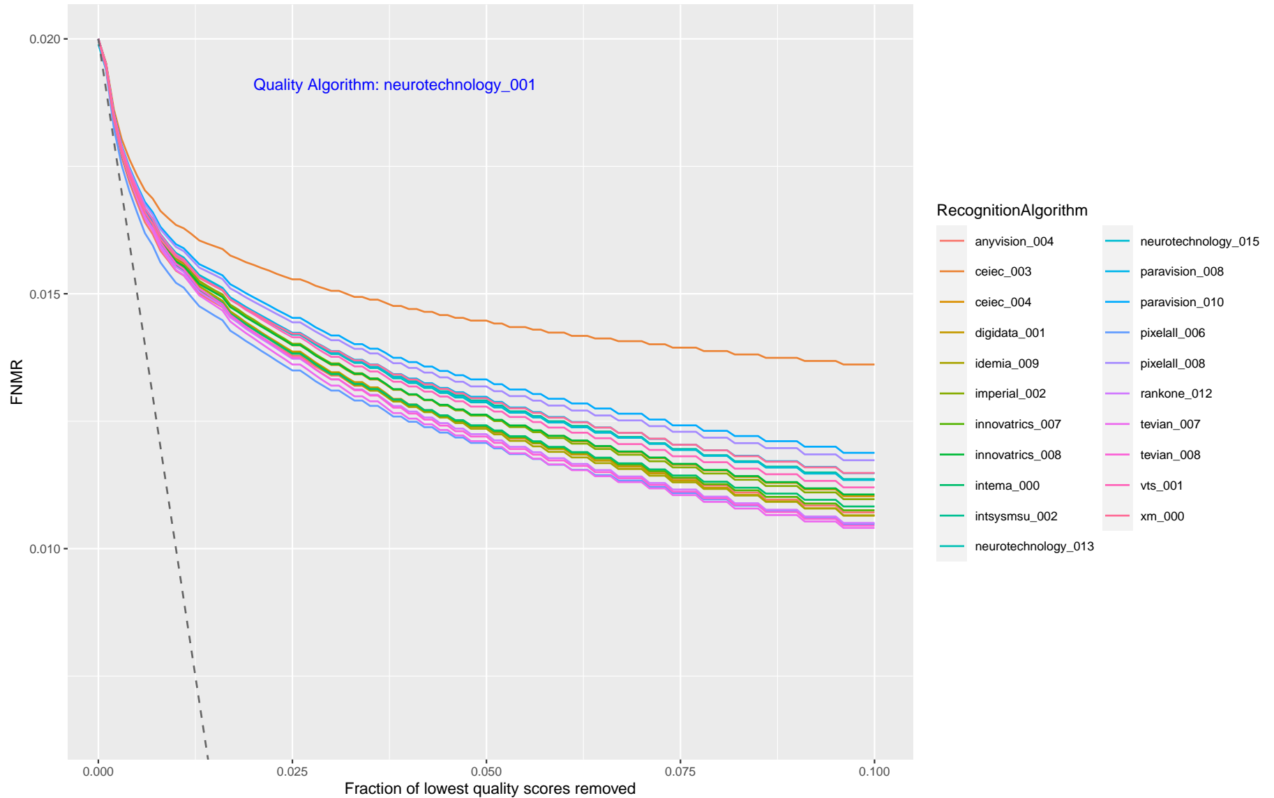
Figure 16: This plot shows FNMR vs. Reject, showing how FNMR reduces when the worst quality data is discarded. Each trace corresponds to a recognition algorithm, and each page corresponds to one quality assessment algorithm. The quality score is from the verification (webcam) border crossing image. A perfect quality algorithm would predict which images are implicated in false non-matches. This is shown by the grey dotted line ( \max((FNMR - x), 0) ). The closer the quality algorithm line is to the perfect line, the better the quality prediction performance is relative to recognition outcomes.
