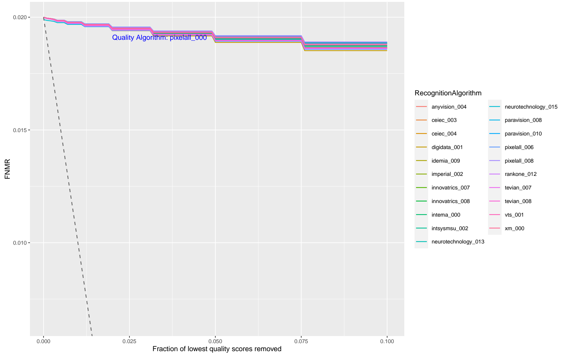
Figure 18: This plot shows FNMR vs. Reject, showing how FNMR reduces when the worst quality data is discarded. Each trace corresponds to a recognition algorithm, and each page corresponds to one quality assessment algorithm. The quality score is from the verification (webcam) border crossing image. A perfect quality algorithm would predict which images are implicated in false non-matches. This is shown by the grey dotted line ( \max((FNMR - x), 0) ). The closer the quality algorithm line is to the perfect line, the better the quality prediction performance is relative to recognition outcomes.
