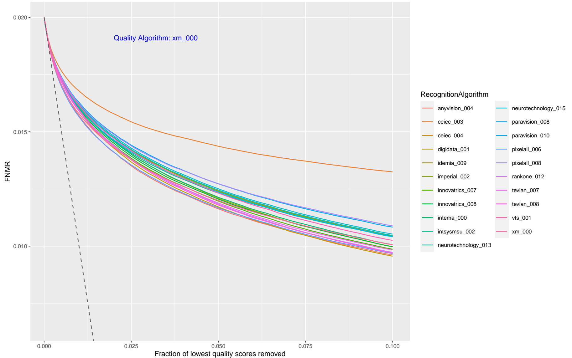
Figure 28: This plot shows FNMR vs. Reject, showing how FNMR reduces when the worst quality data is discarded. Each trace corresponds to a recognition algorithm, and each page corresponds to one quality assessment algorithm. The quality score is from the verification (webcam) border crossing image. A perfect quality algorithm would predict which images are implicated in false non-matches. This is shown by the grey dotted line ( \max((FNMR - x), 0) ). The closer the quality algorithm line is to the perfect line, the better the quality prediction performance is relative to recognition outcomes.
