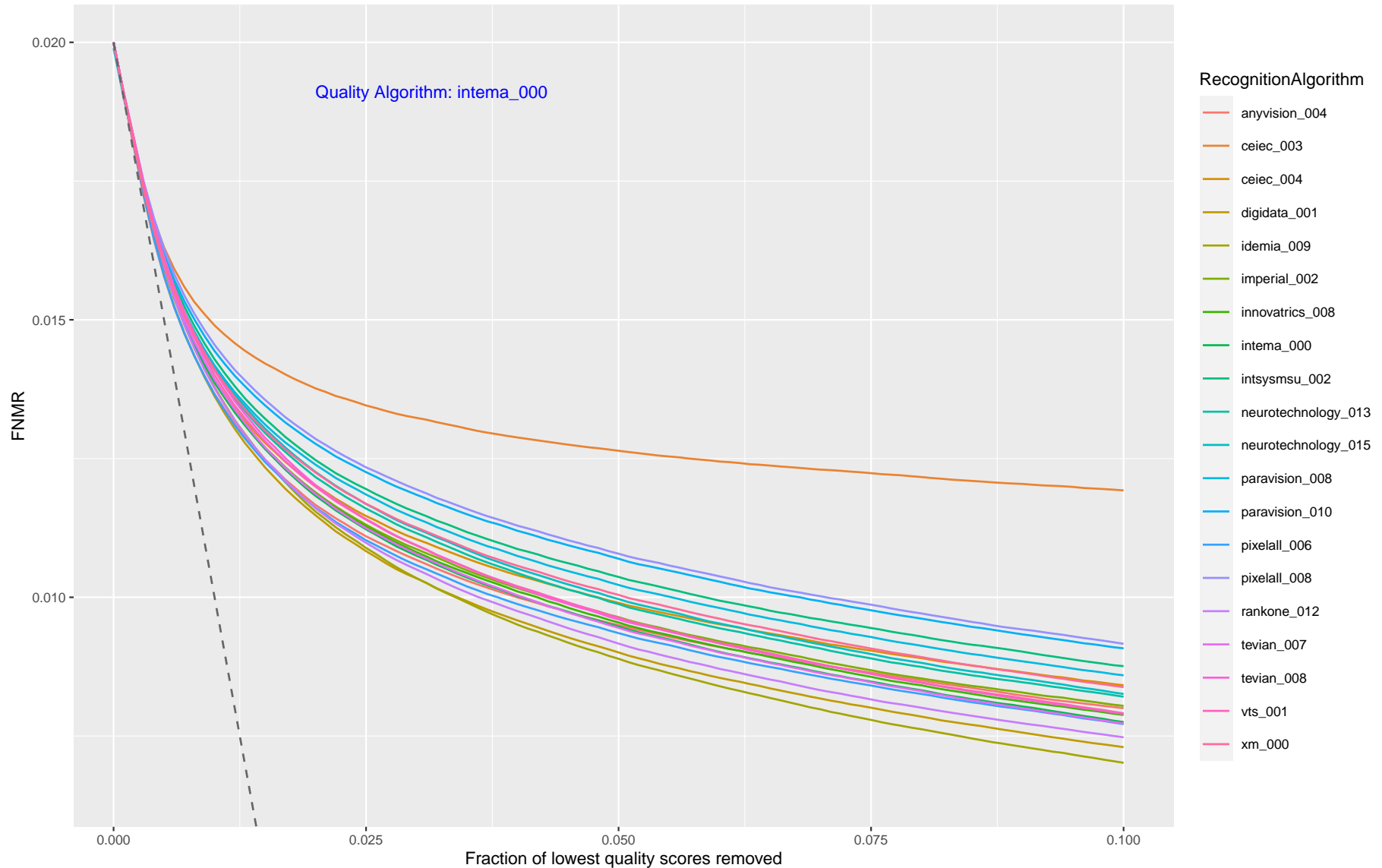
Figure 14: This plot shows FNMR vs. Reject, showing how FNMR reduces when the worst quality data is discarded. Each trace corresponds to a recognition algorithm, and each page corresponds to one quality assessment algorithm. The quality score is from the verification (webcam) border crossing image. A perfect quality algorithm would predict which images are implicated in false non-matches. This is shown by the grey dotted line ( \max((FNMR - x), 0) ). The closer the quality algorithm line is to the perfect line, the better the quality prediction performance is relative to recognition outcomes.
