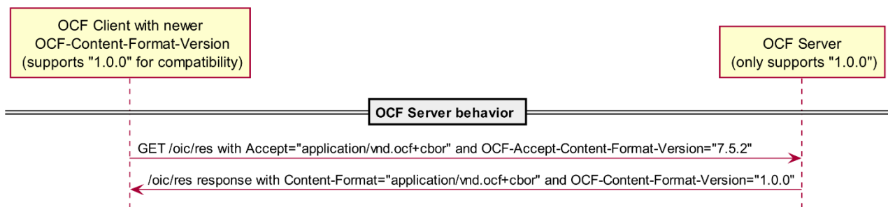
Figure 33 – Content-Format Policy for backward compatible OCF Clients negotiating lower OCF Content-Format-Version
