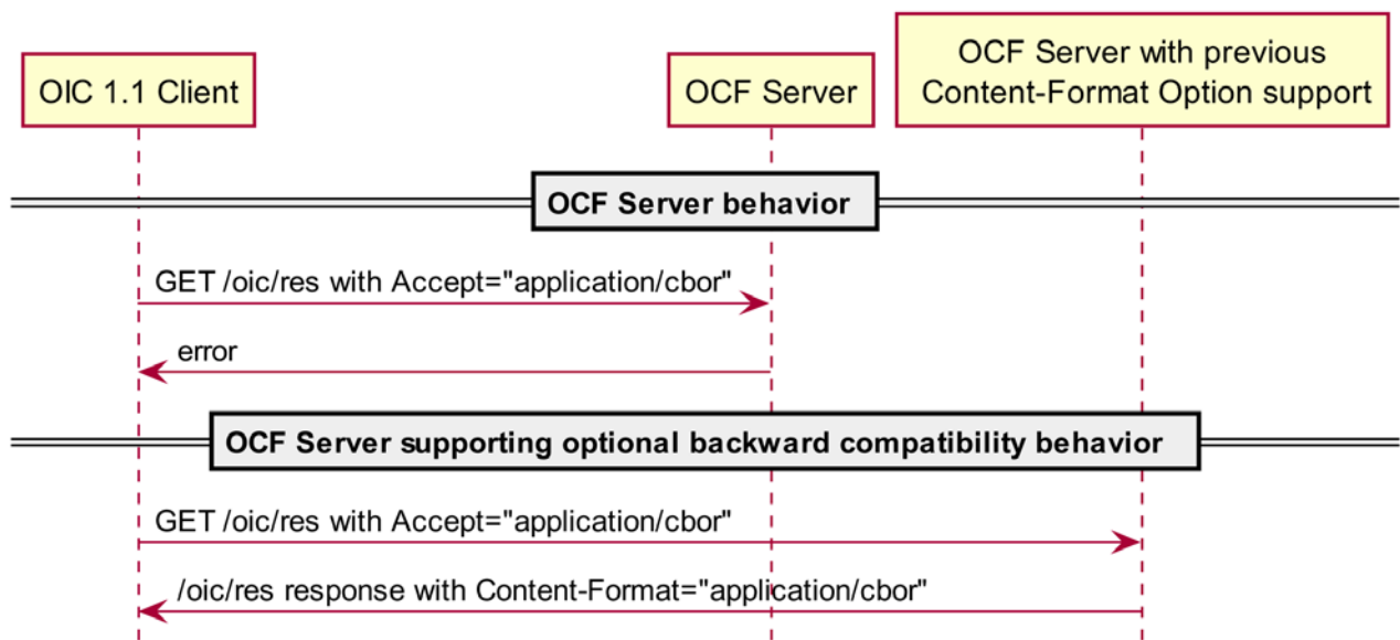
4344 Figure 31 – Content-Format Policy for OCF Servers supporting error responses and 4345 backward compatibility responses
