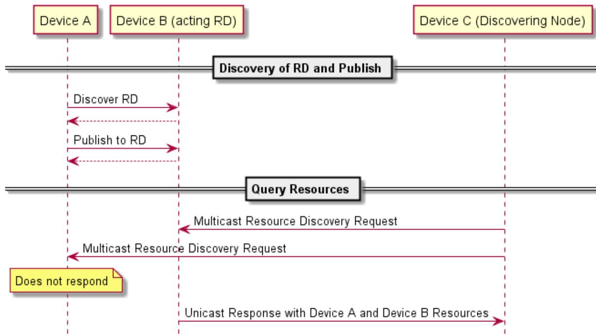
Figure 18 – RD discovery and RD supported query of Resources support
