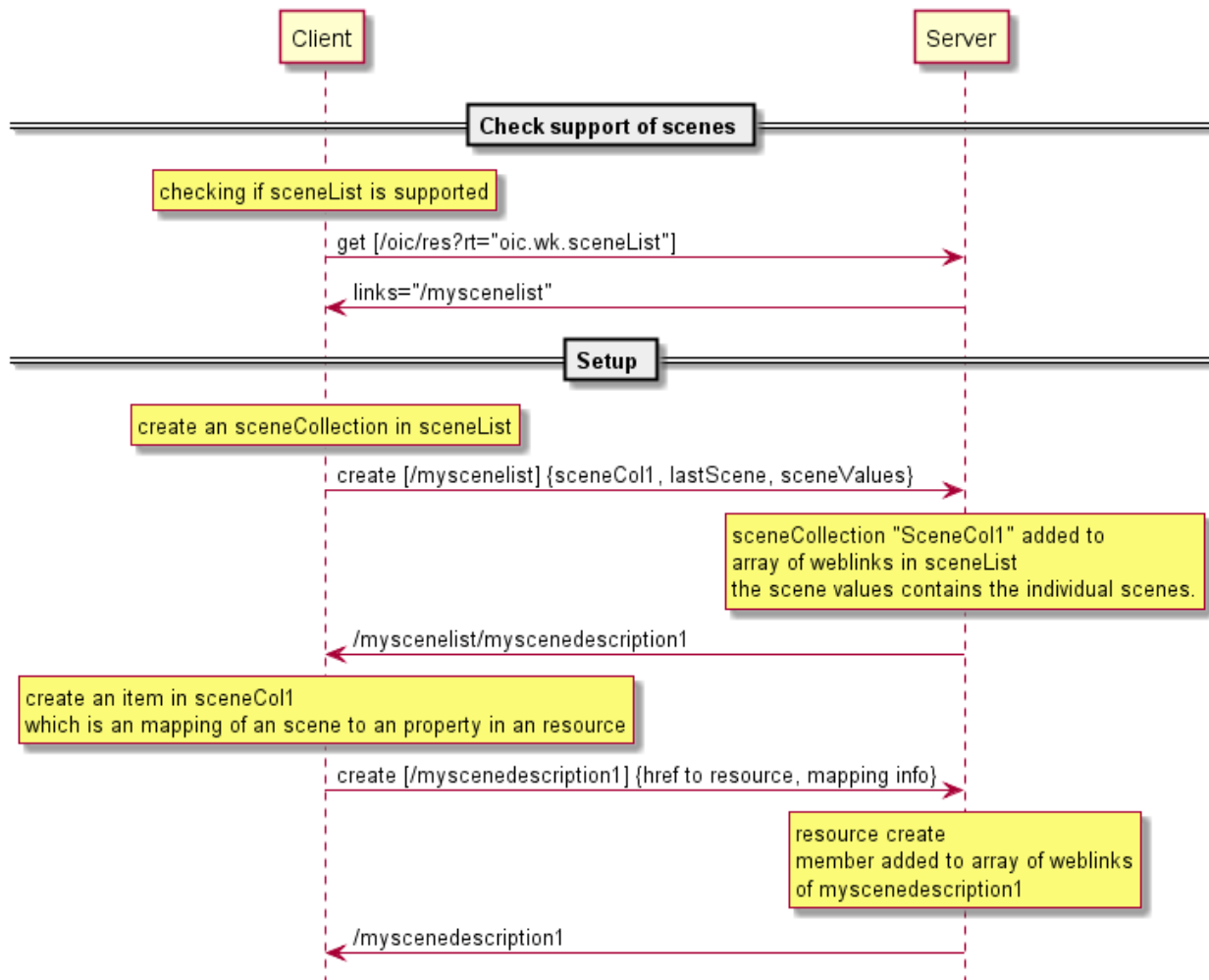
3961 Figure 26 – Interactions to check Scene support and setup of specific Scenes
