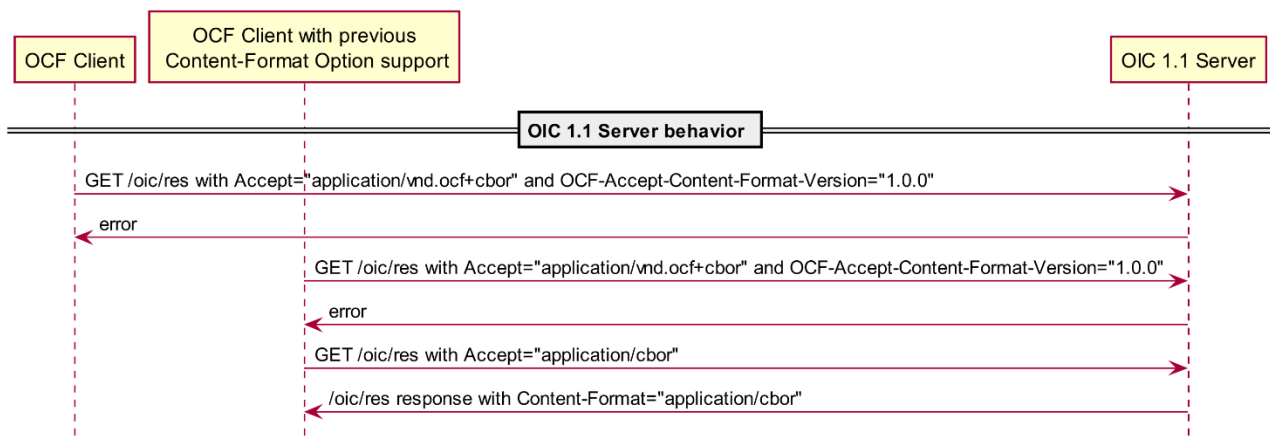
Figure 32 – Content-Format Policy for OCF Clients supporting error responses and backward compatibility responses
