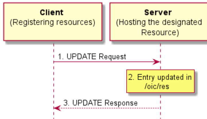
Figure 15 – Resource based discovery: Information publication process
