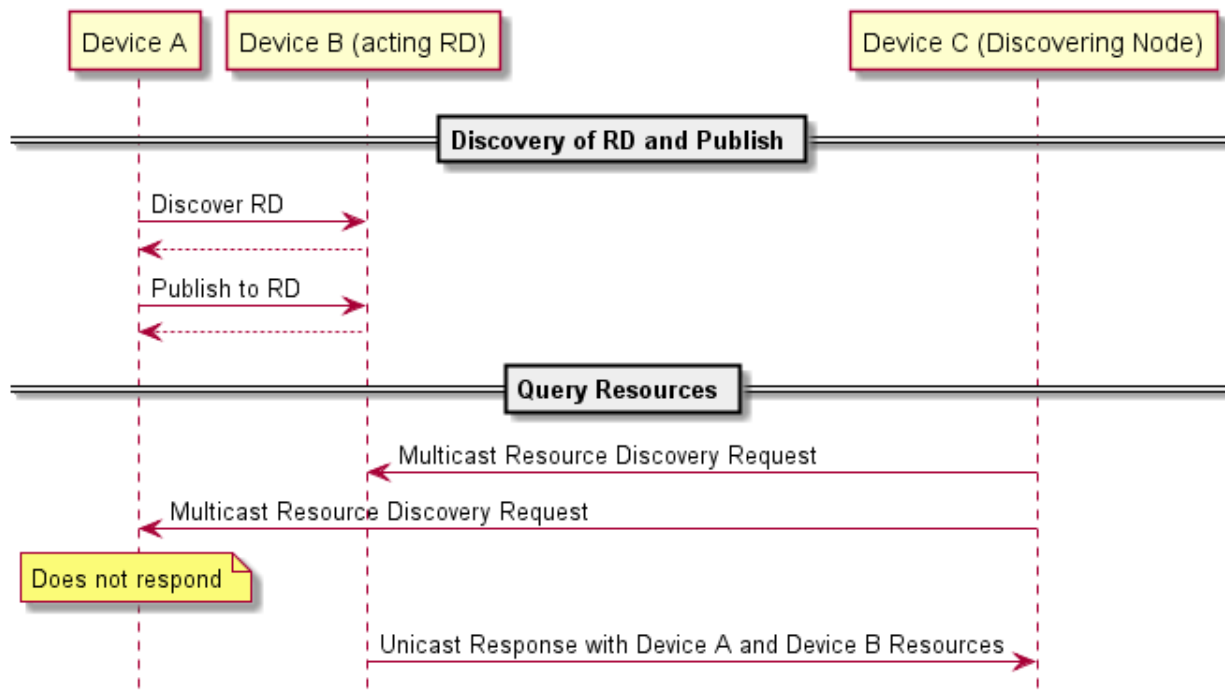
Figure 18 – RD discovery and RD supported query of Resources support
