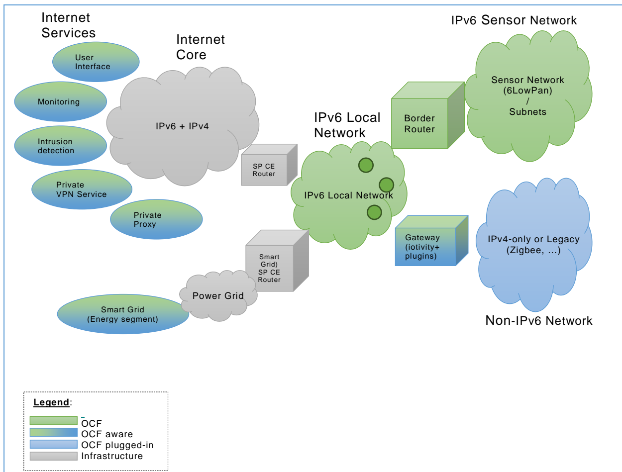
Figure 14 – High Level Network & Connectivity Architecture
