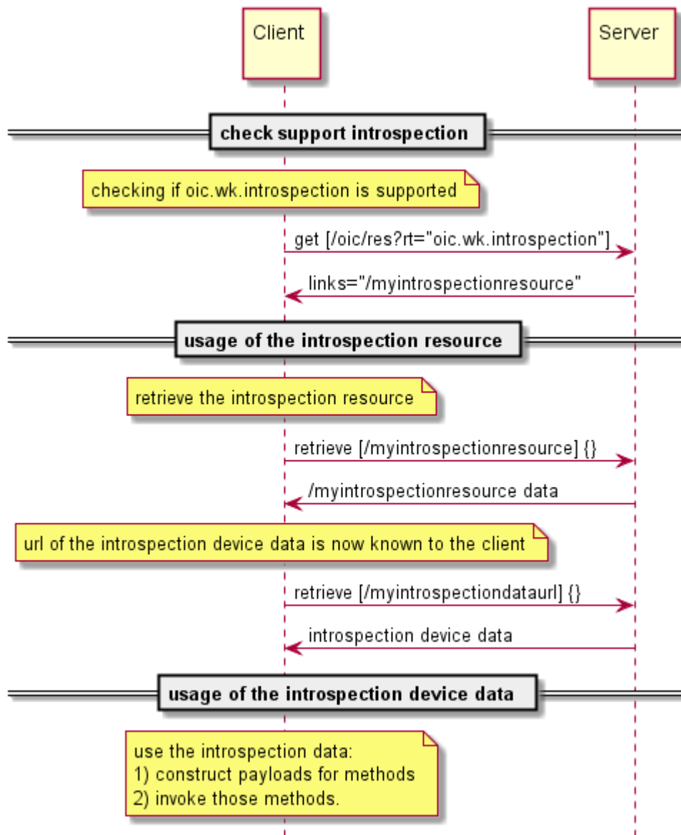
Figure 28 – Interactions to check Introspection support and download the Introspection Device Data.
