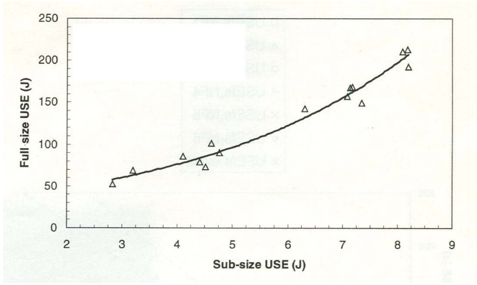
Figure 19 - Exponential correlation between sub-size and full-size USE values for KLST specimens [10].
