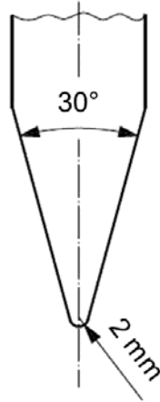
Figure 3 – 2-mm striker used for performing impact tests on KLST specimens.
