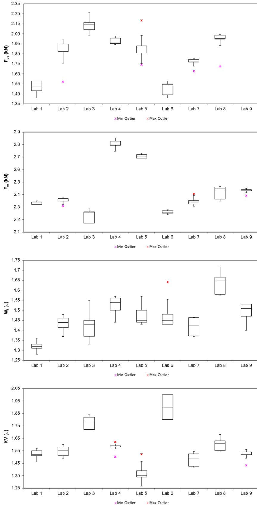
Figure 7 – “Box-and-whiskers” plots for the low-energy specimens.
