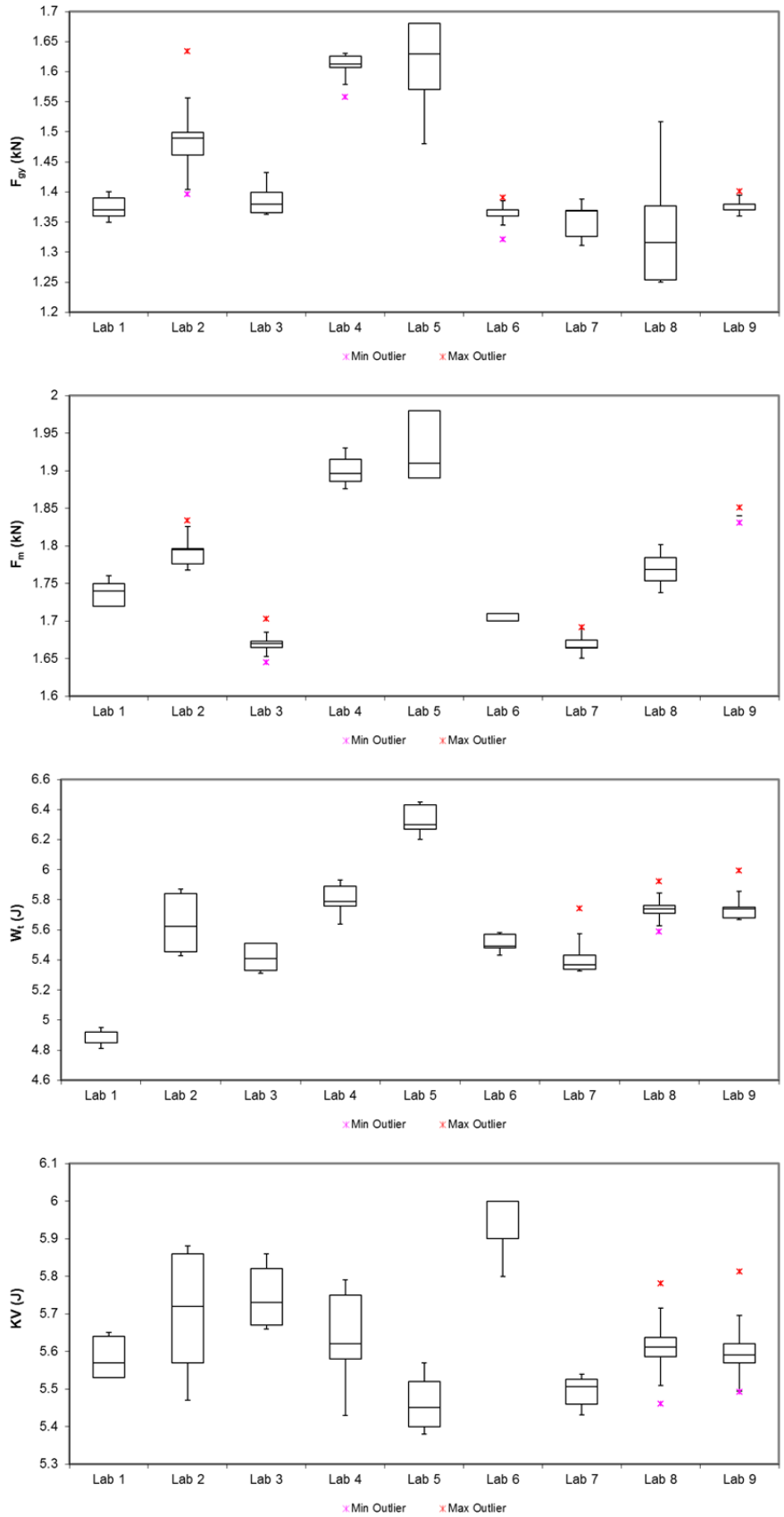
Figure 8 – “Box-and-whiskers” plots for the high-energy specimens.
