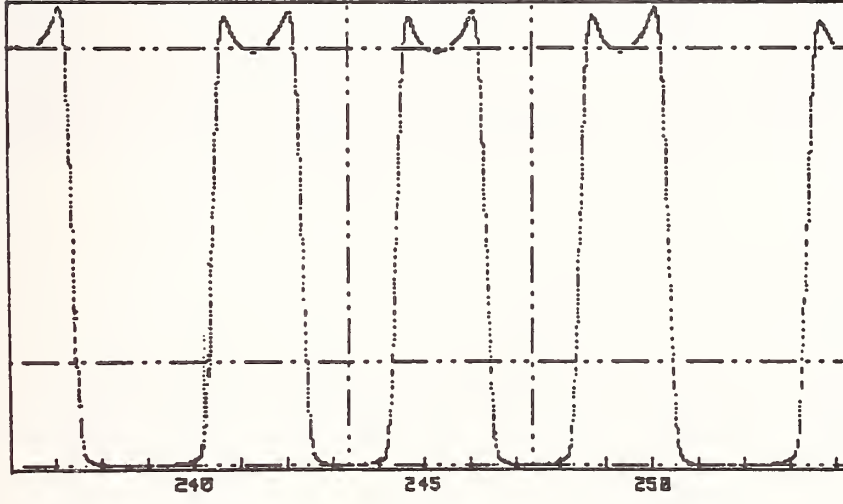
Figure 7. Samples of optical profiles (measured light intensity versus position) displayed on the computer screen during the calibration process. The vertical axes are relative light intensity and the horizontal axes are position in micrometers. The horizontal lines are fiducials marking the relative intensity levels of the clear and coated areas and the threshold.
