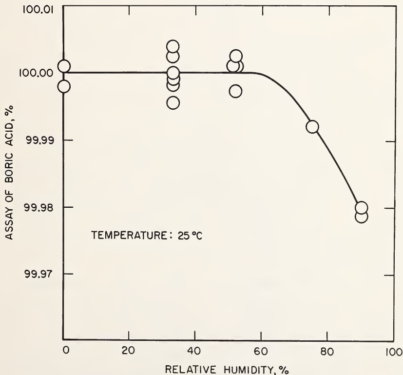
Figure 7. Effect of the Humidity of the Environment on the Assay of Boric Acid.
