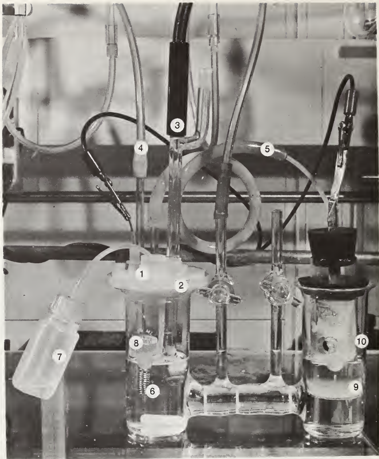
Figure 3. Coulometric Titration Cell for Precise Acidimetry.
