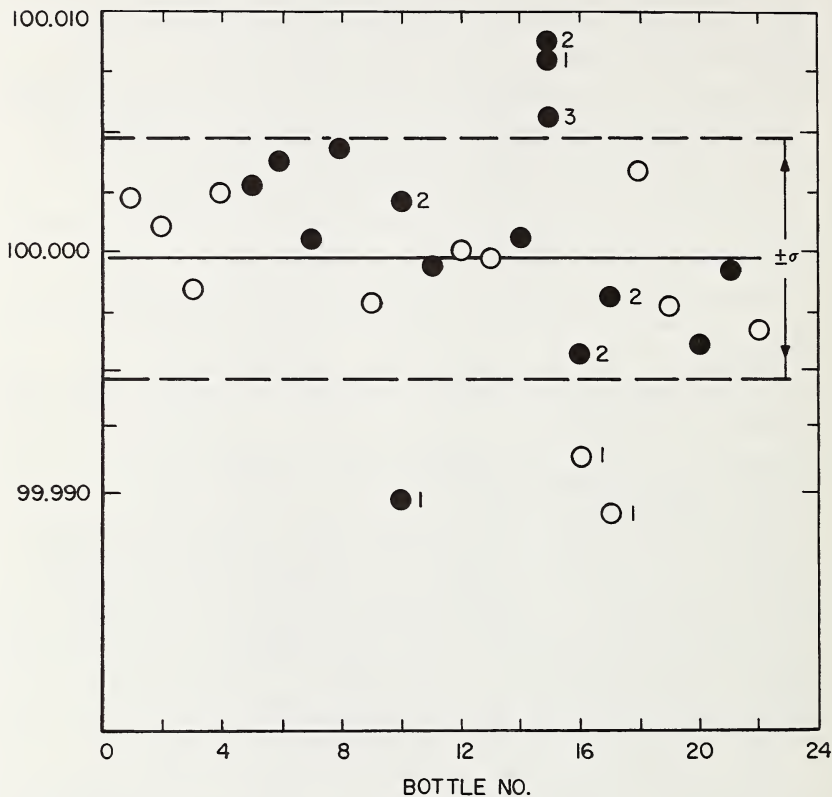
Figure 4. Homogeneity of SRM 951, Boric Acid.
