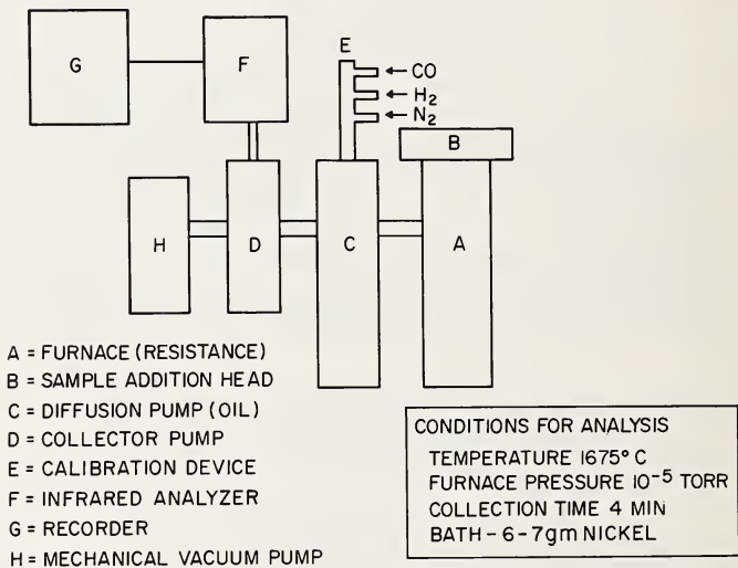
Figure 2. Schematic diagram of vacuum-fusion-CO infrared apparatus.
