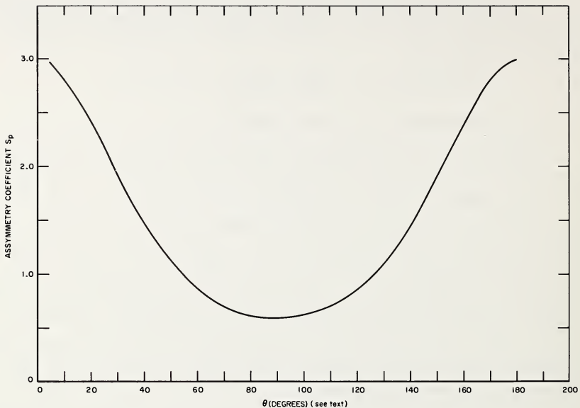
Figure 6. Peak intensity asymmetry for the {}^{\pm}3/2 \rightarrow {}^{\pm}1/2 doublet in iron compounds as a function of the angle between the electric field gradient and the incident radiation.
