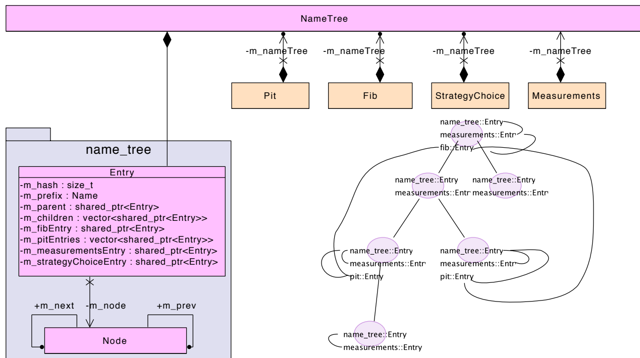
Figure 8: NameTree overview
