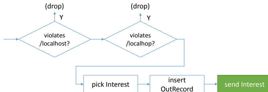
Figure 12: Outgoing Interest pipeline
