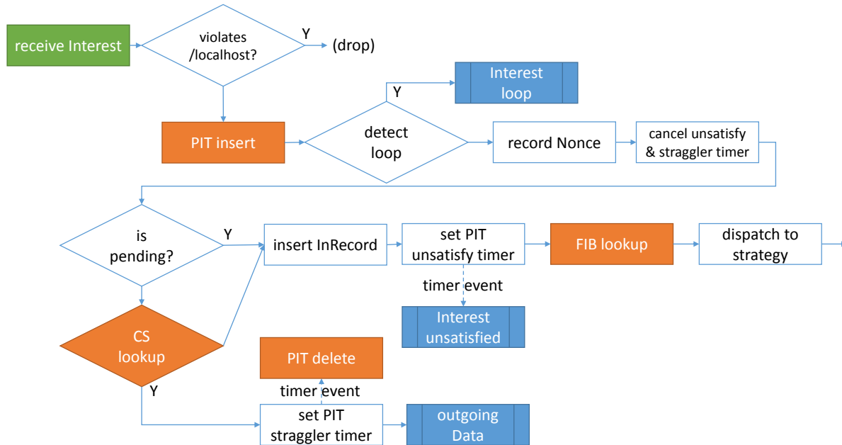
Figure 11: Incoming Interest pipeline
