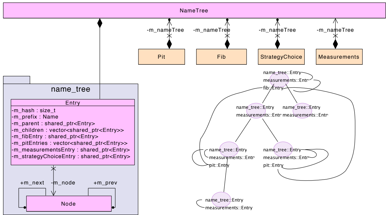
Figure 8: NameTree overview
