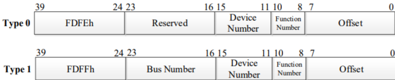
Figure 5. Standard access address of the PCI configuration
