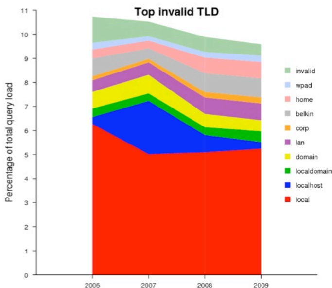
Figure 1. Traffic for invalid TLDs (2009)
