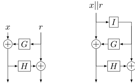
(b) OAEP( x; r ) (left) and RInj( x; r ) = AOAEP( x; r ) (right); x is the input, r is uniformly random.
