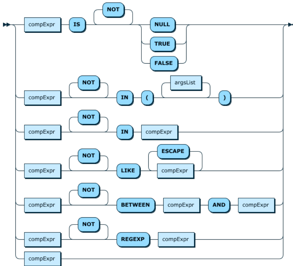
Figure 12.28 ilriExpr
