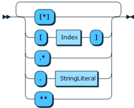
Figure 11.34 DocPath
