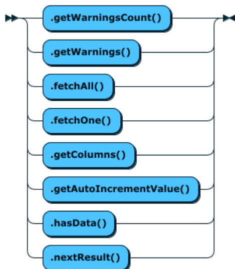
Figure 11.23 SqlResult
