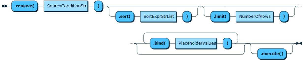
Figure 11.12 CollectionRemoveFunction
