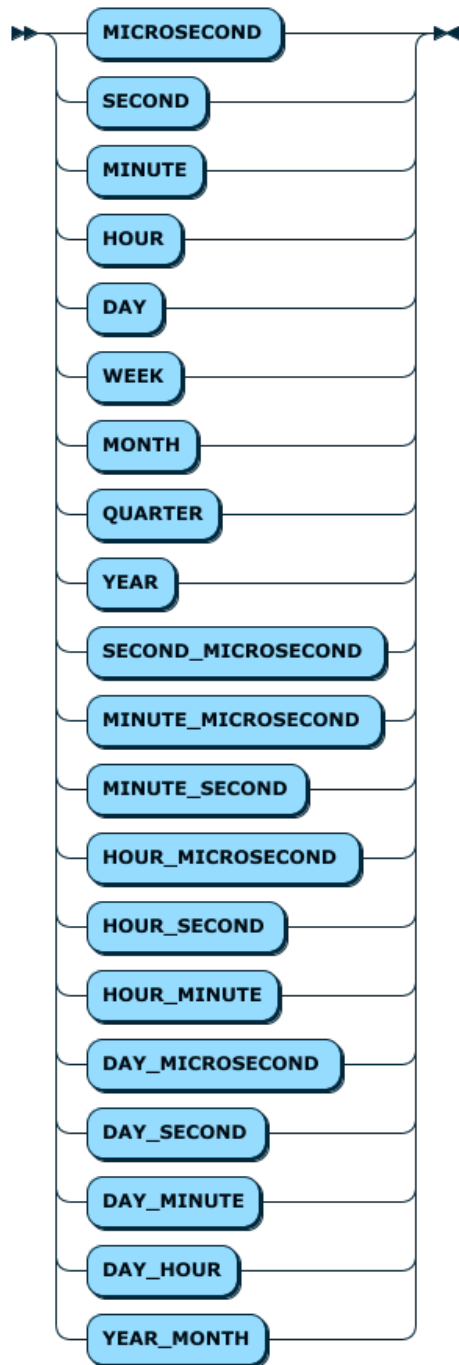
Figure 12.20 INTERVAL_UNIT
