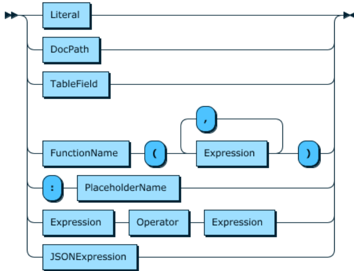
Figure 11.36 Expression
