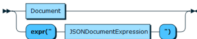
Figure 11.41 DocumentOrJSON
