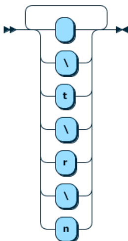
Figure 12.37 WS
