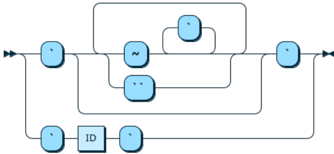
Figure 12.35 QUOTED_ID
