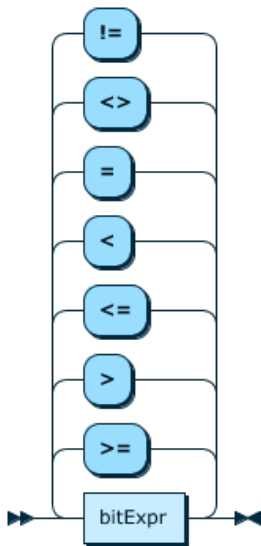
Figure 12.27 compExpr
