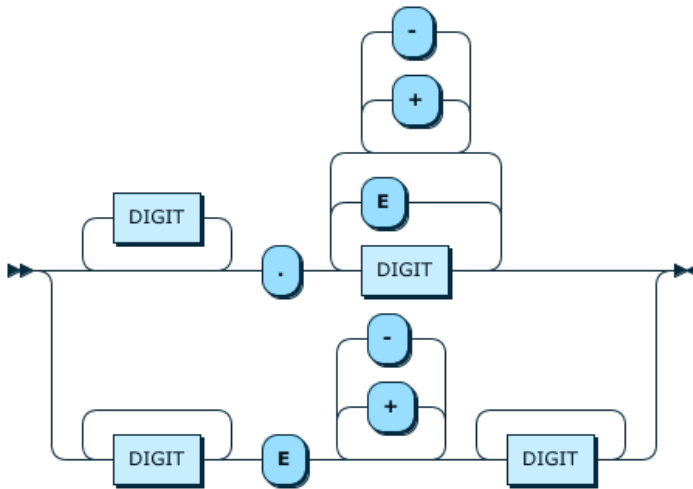
Figure 12.33 FLOAT
