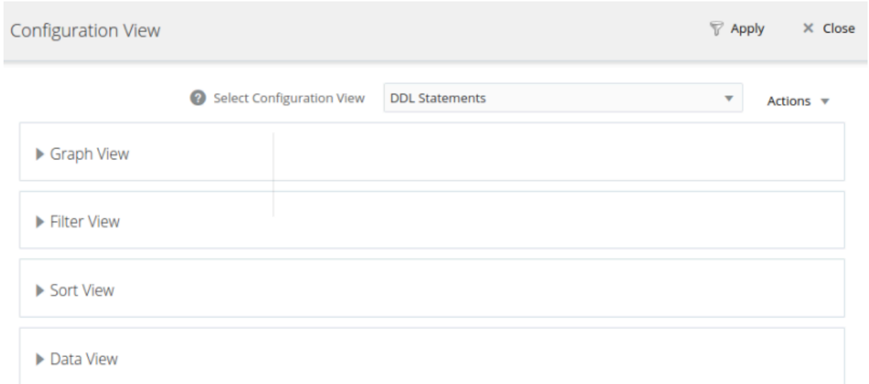
Figure 32.7 Configuration View
