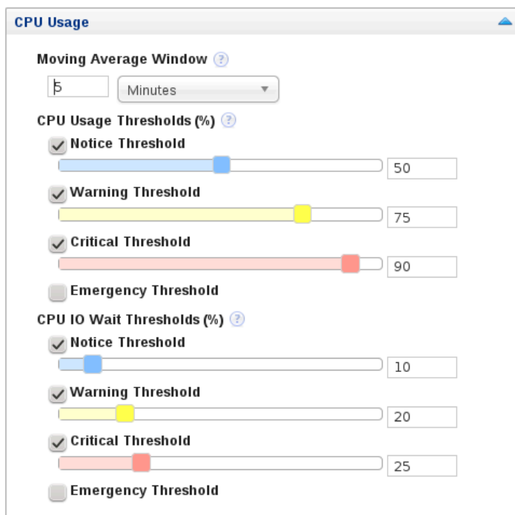
Figure 21.4 CPU Usage
