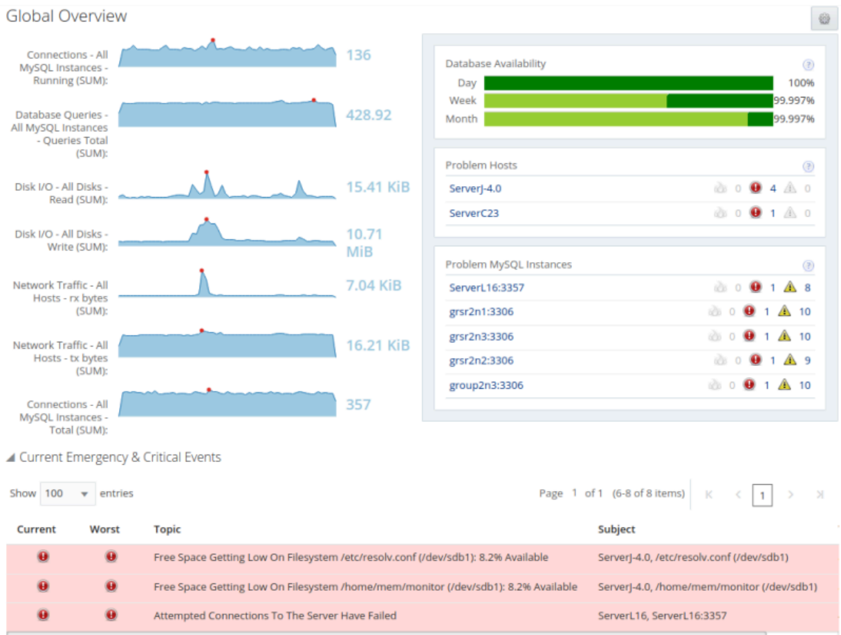
Figure 25.1 Global Overview
