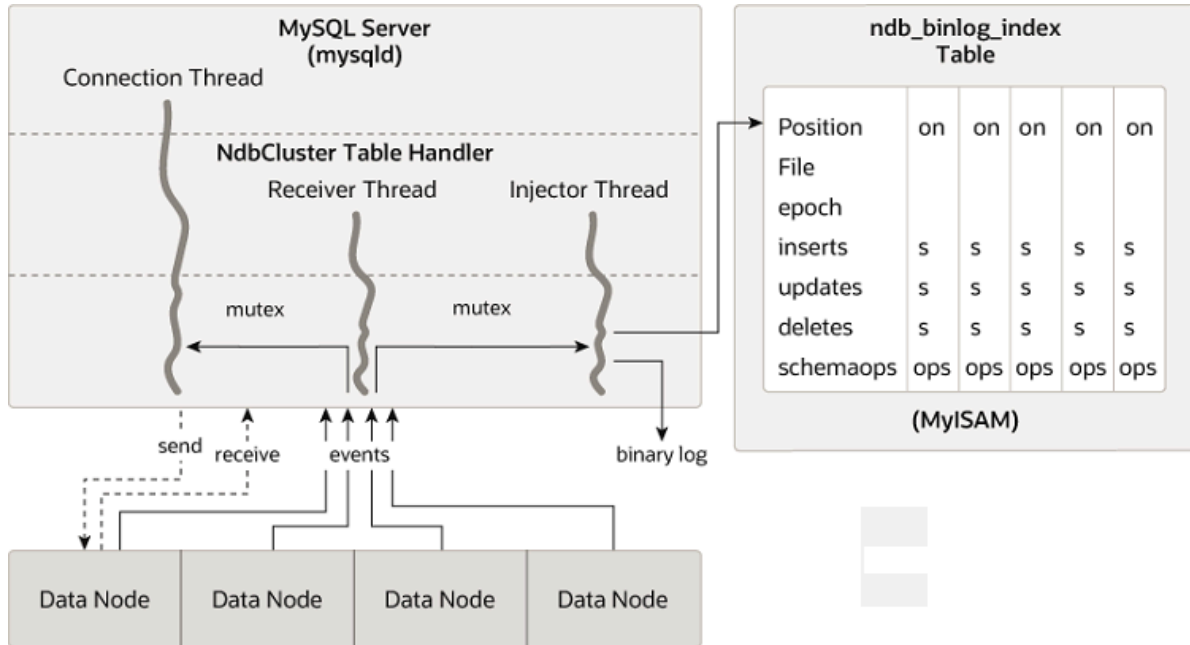
Figure 7.4 The Replication Source Cluster
