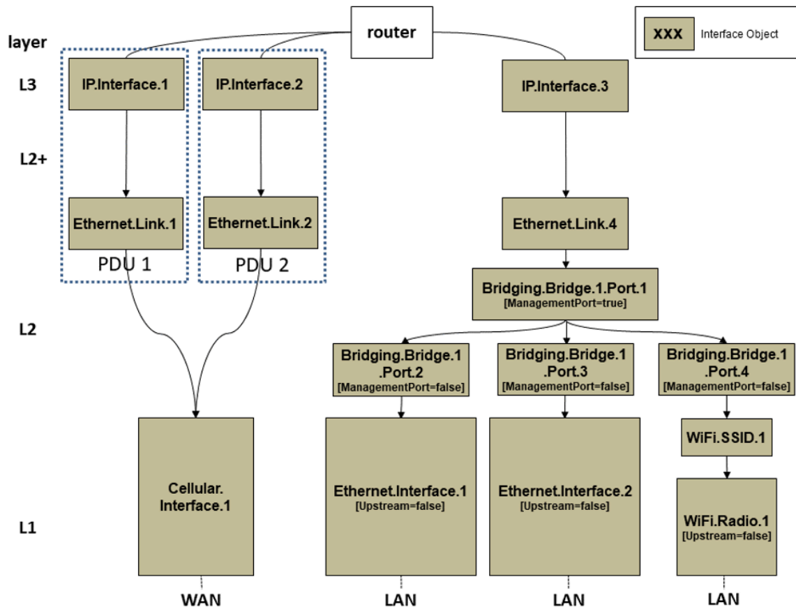
Figure 81: Cellular access only example
