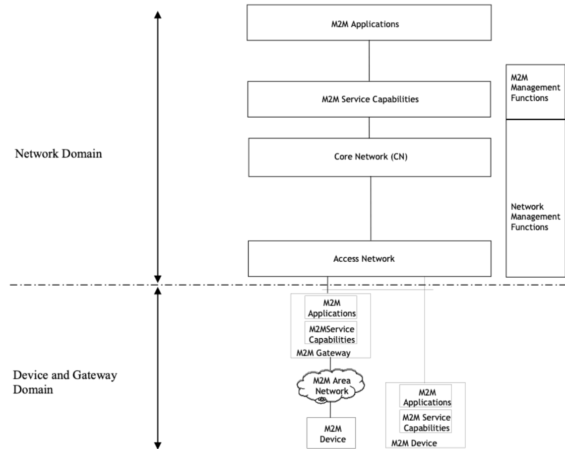
Figure 46: ETSI High Level Functional Architecture
