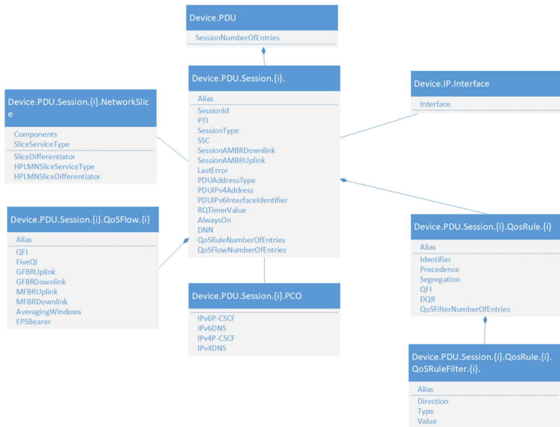
Figure 84: Device.PDU objects
