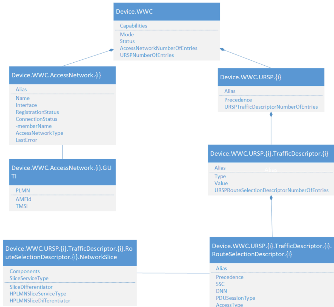
Figure 83: Device.WWC objects
