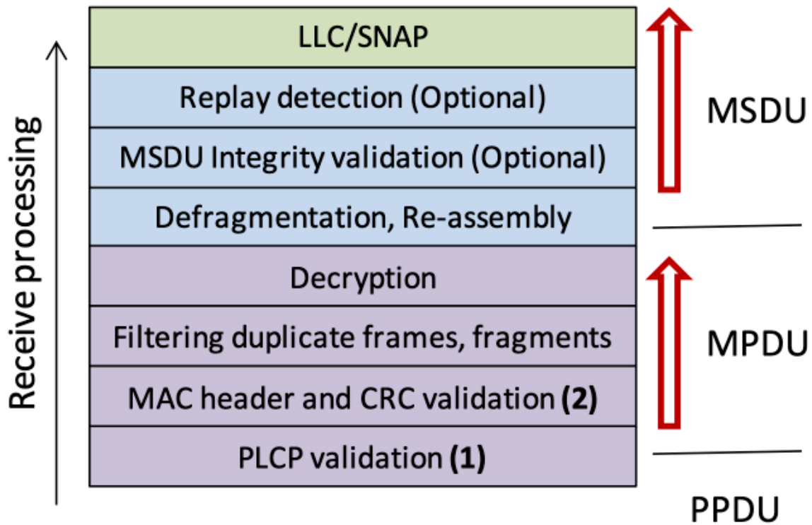
Figure 33: WiFi functions within layers
