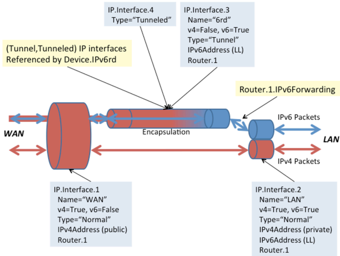
Figure 39: Sample 6rd Routing and Forwarding
