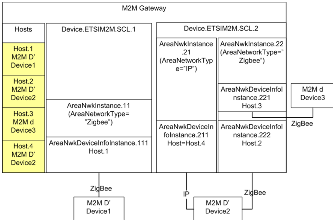
Figure 50: Example M2M Network
