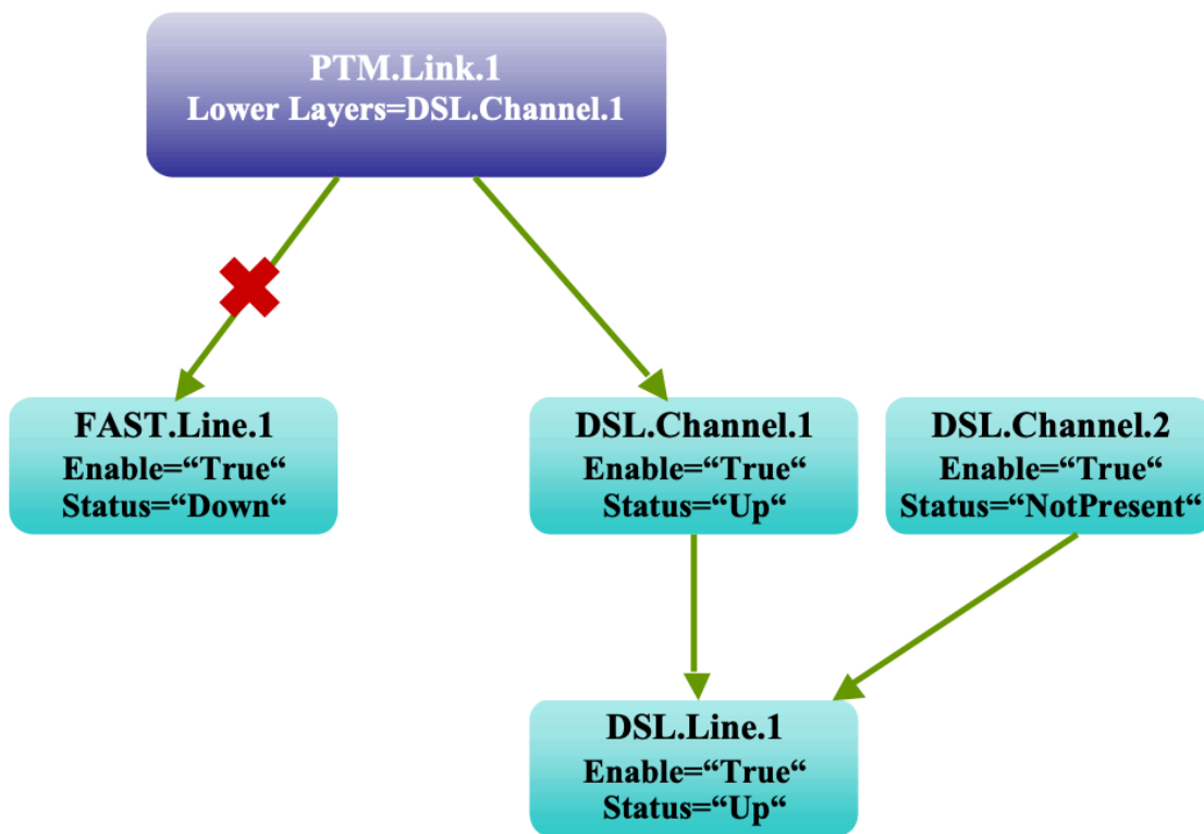
Figure 66: PTM Link for DSL mode Line
