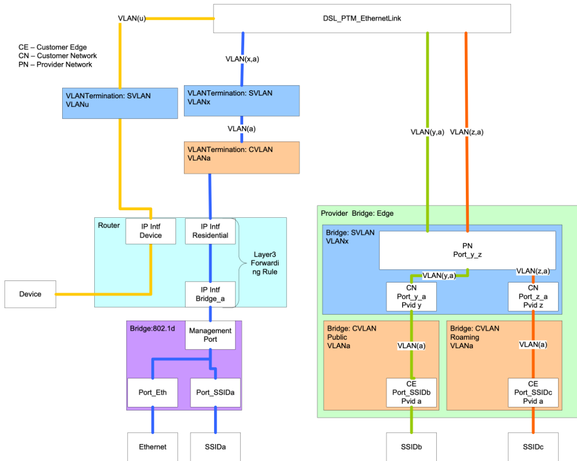
Figure 54: Provider Bridge Components
