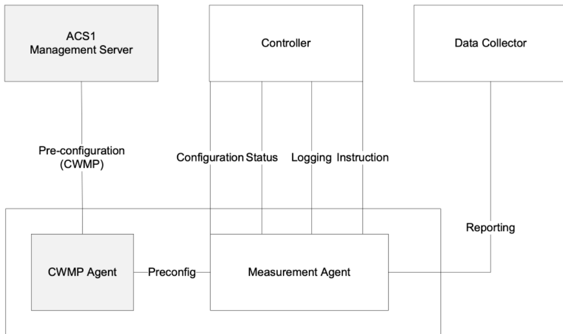
Figure 73: CWMP for Pre-configuration
