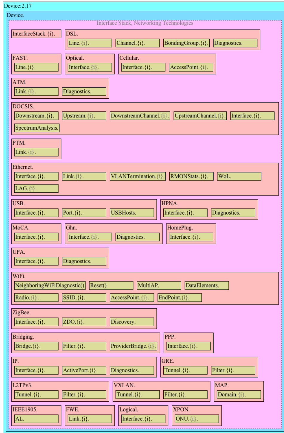
Figure 4: Device:2 Data Model Structure – Common Interface Stack and Networking Technologies
