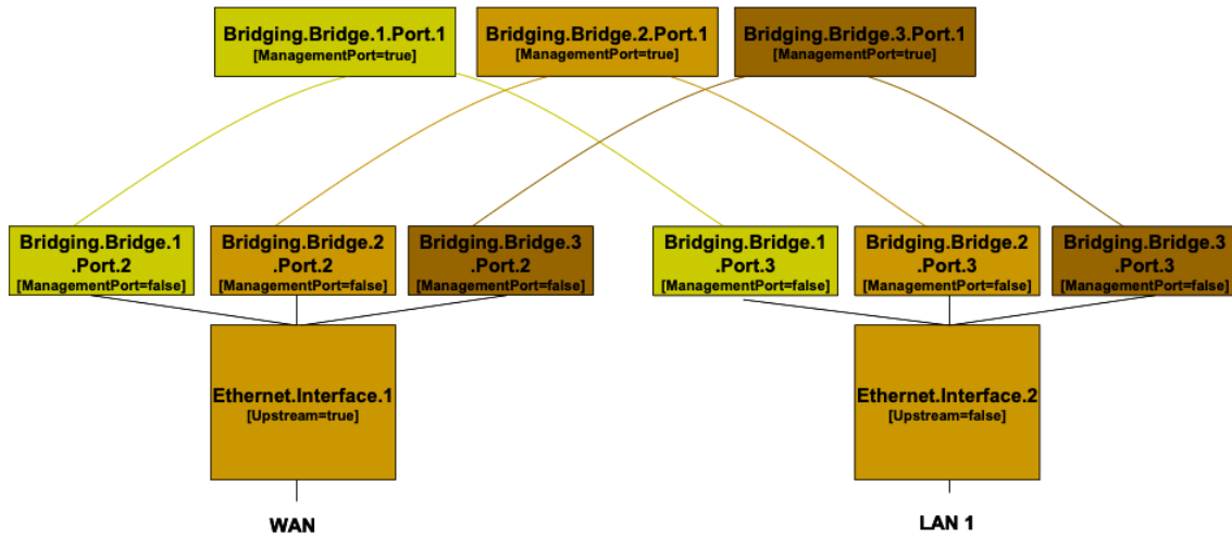
Figure 32: Bridge 1,2,3 model
