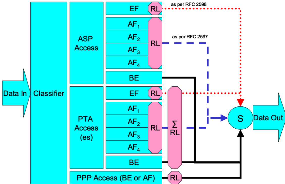
Figure 24: Queuing and Scheduling Example for RG
