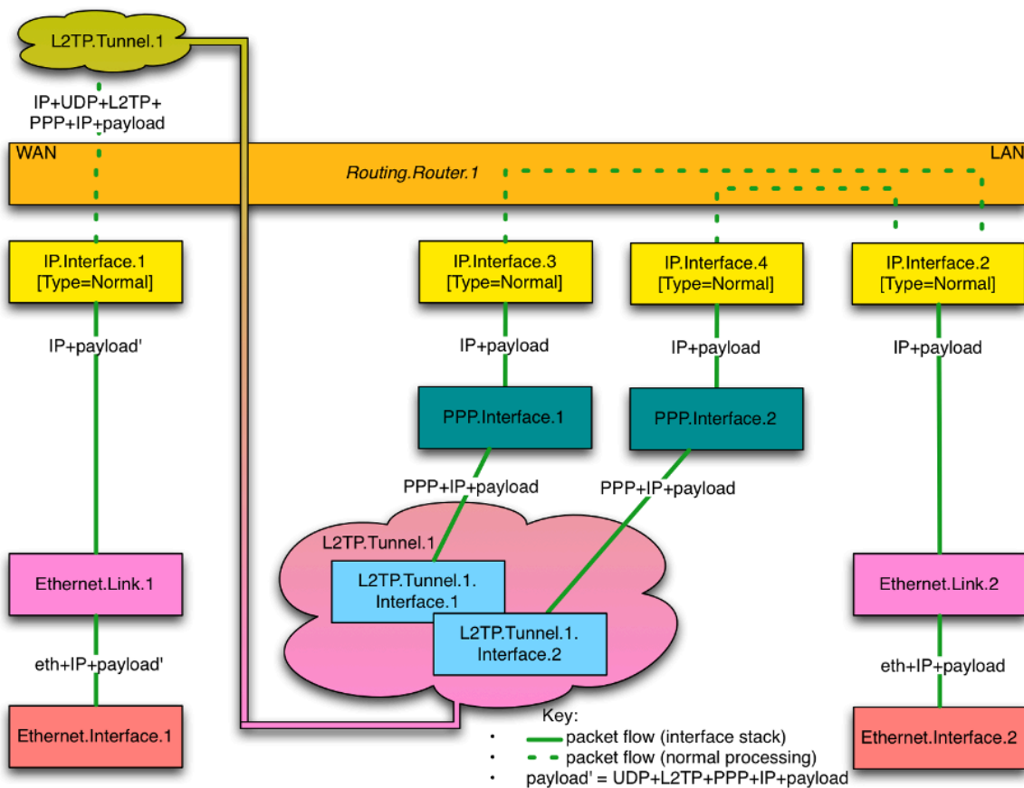
Figure 22: L2TP Interface Stack Example
