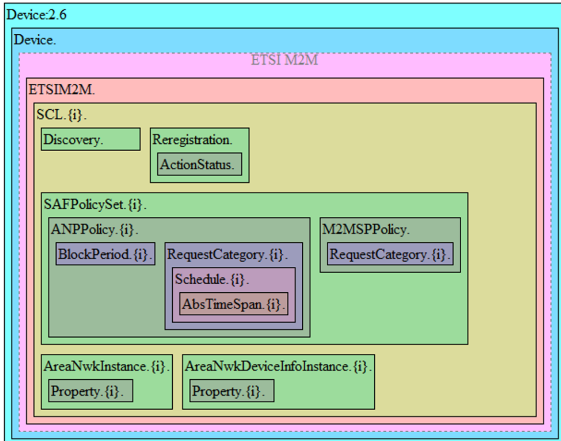
Figure 52: ETSI M2M Data Model Structure
