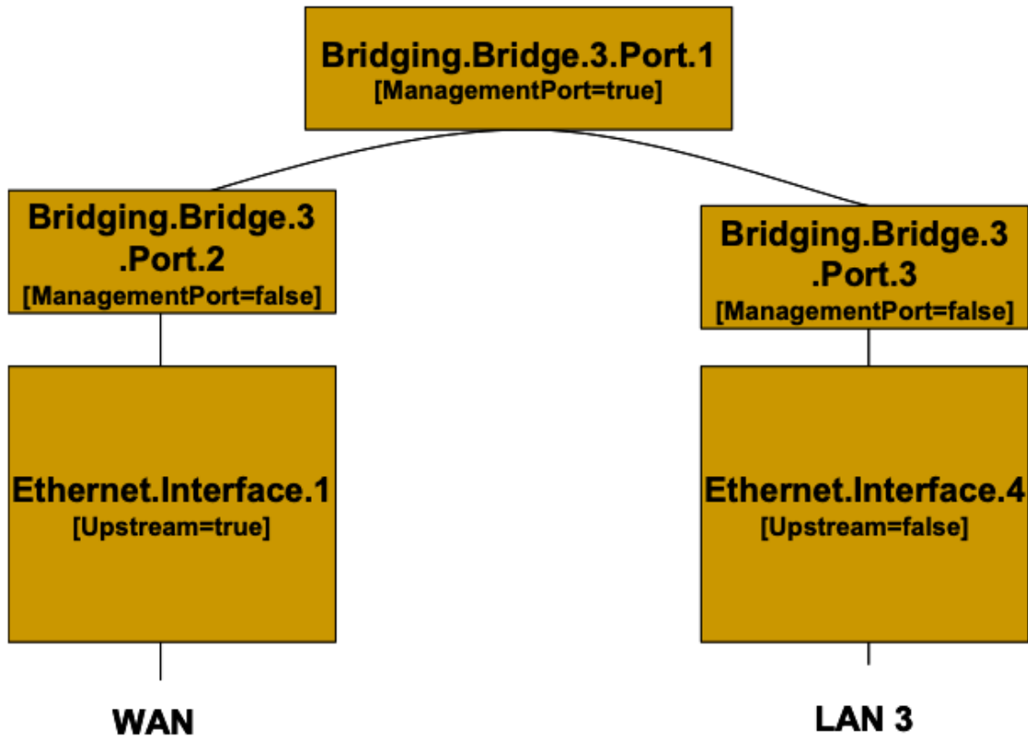
Figure 28: Bridge 3 model
