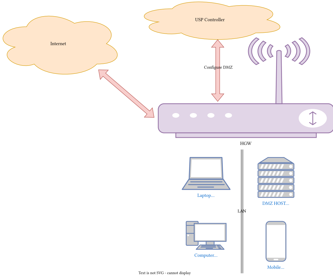
Figure 42: DMZ example
