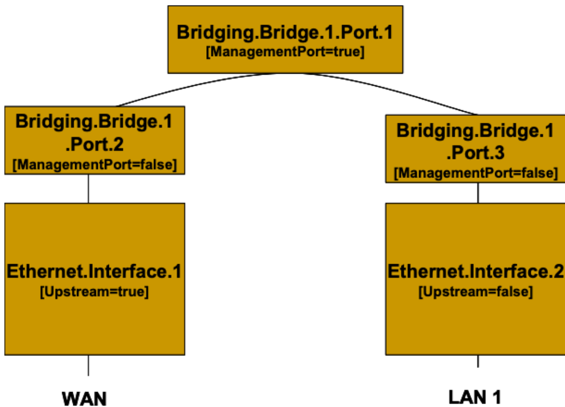
Figure 26: Bridge 1 model
