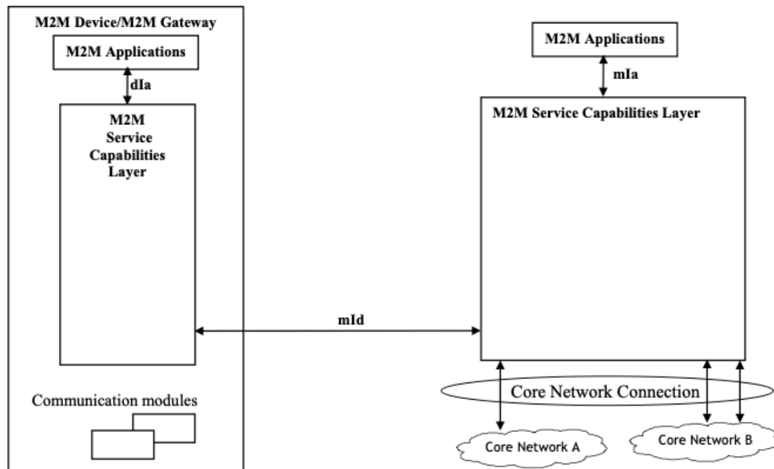
Figure 47: M2M SCL Functional Architecture Framework
