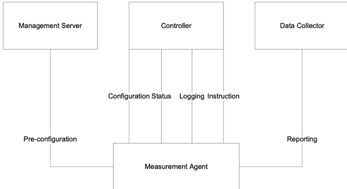
Figure 72: LMAP Framework
