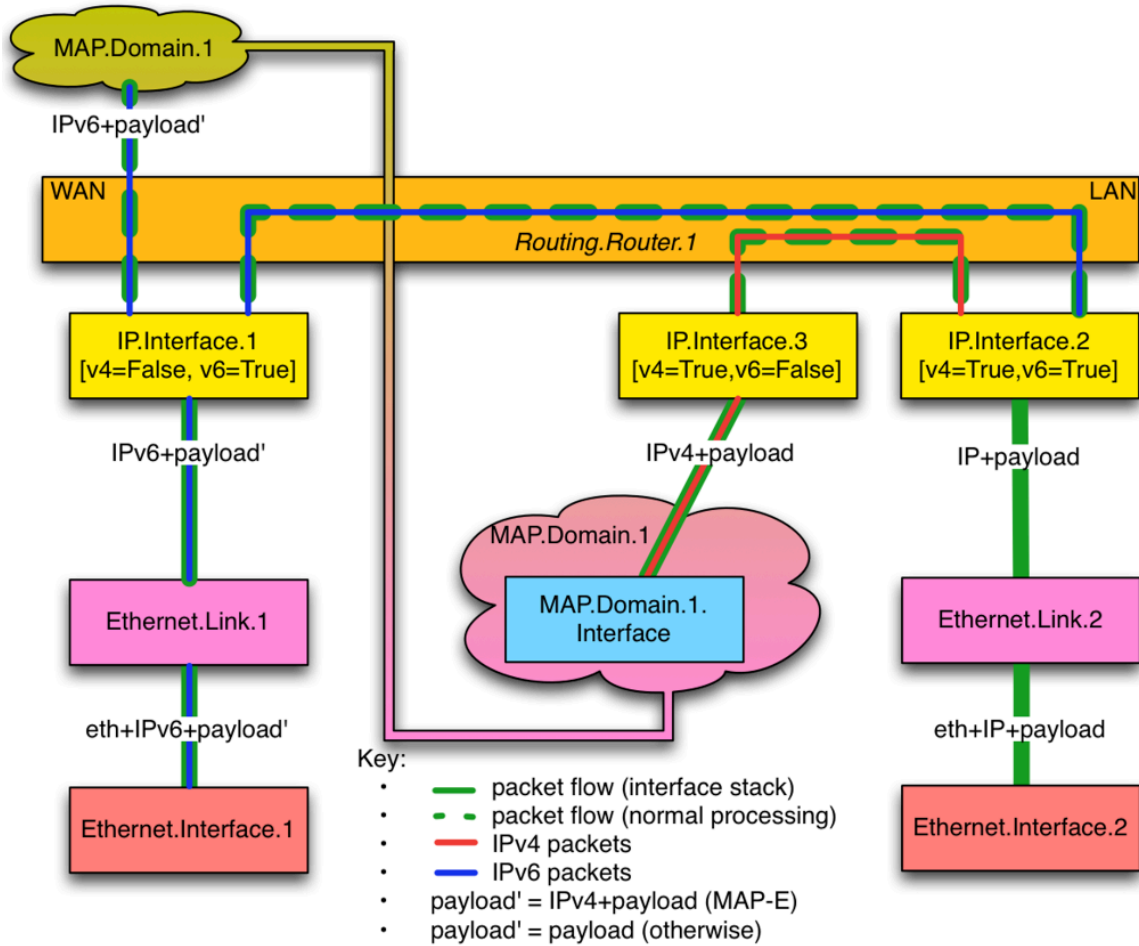
Figure 65: Sample MAP Routing and Forwarding (Interface Stack)
