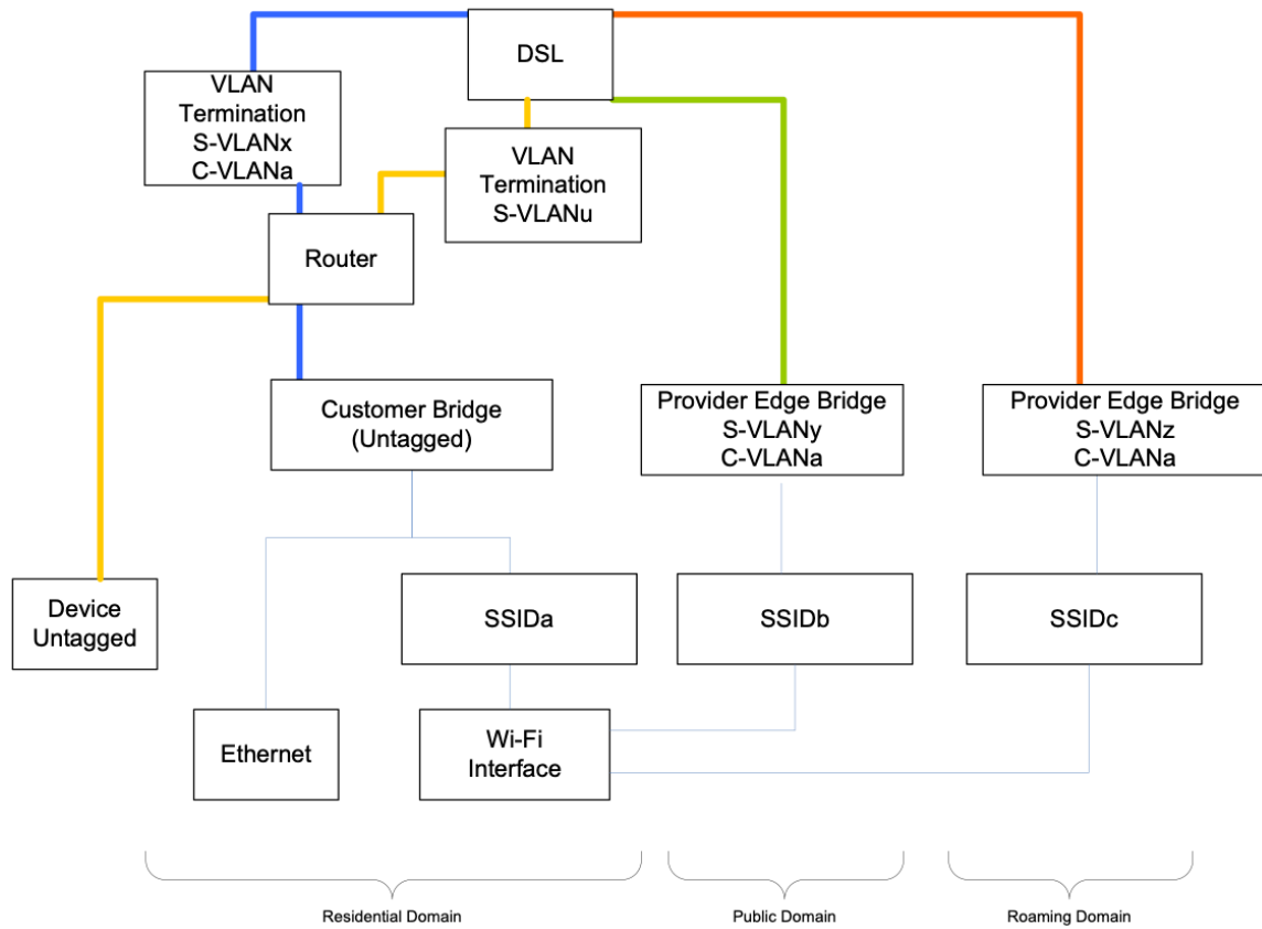
Figure 53: Provider Bridge Scenarios
