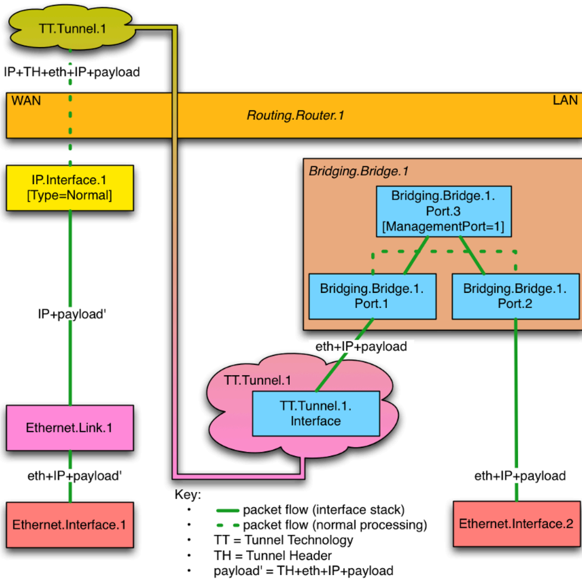
Figure 23: General Layer 2 Tunneling Interface Stack
