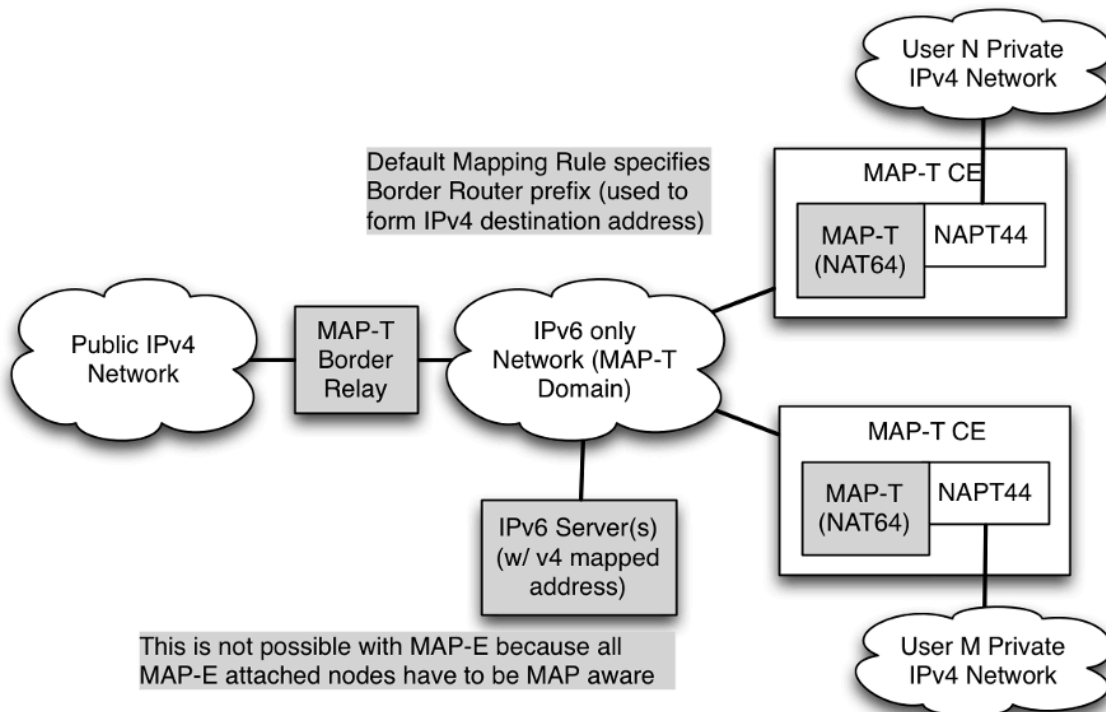
Figure 63: MAP-T Architecture
