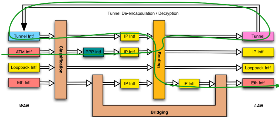
Figure 19: Sample Flow of Downstream Tunneled Traffic through the Device
