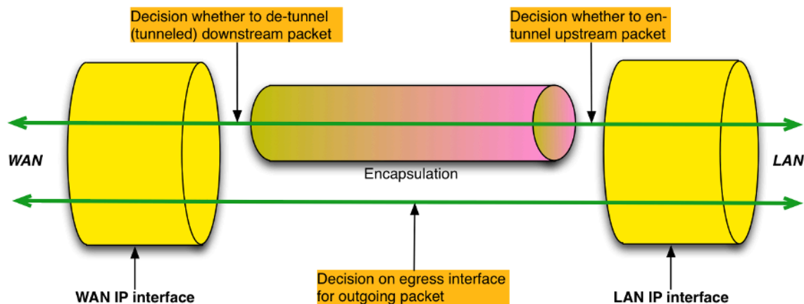
Figure 16: Tunneling Overview
