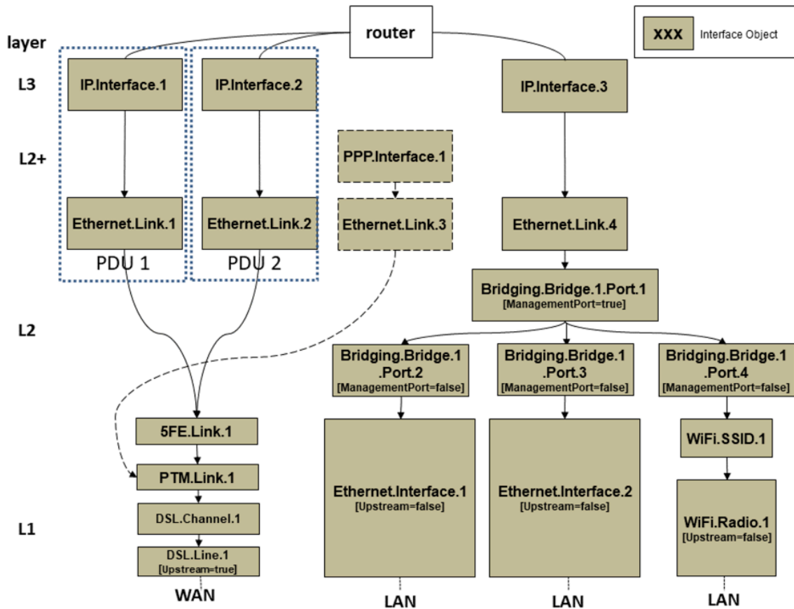
Figure 80: Fixed access only example
