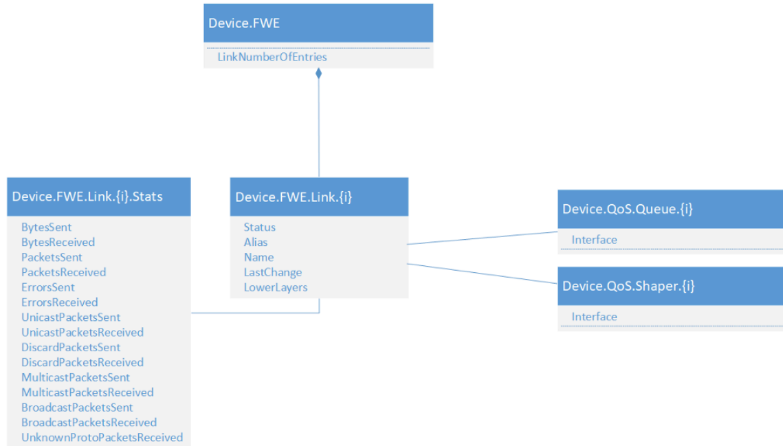
Figure 85: Device.FWE objects
