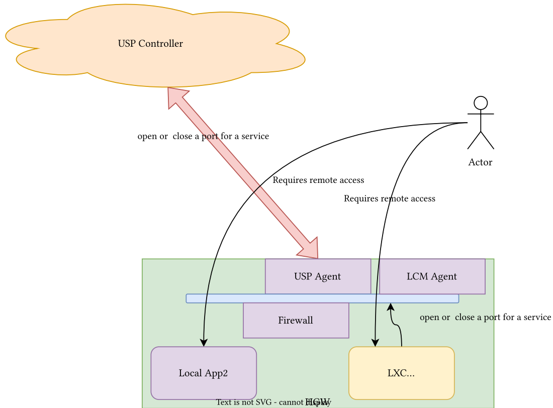
Figure 44: Local service example
