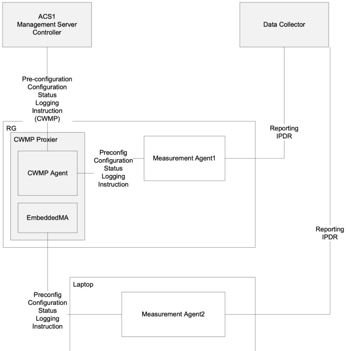
Figure 75: CWMP Proxy Device Deployment
