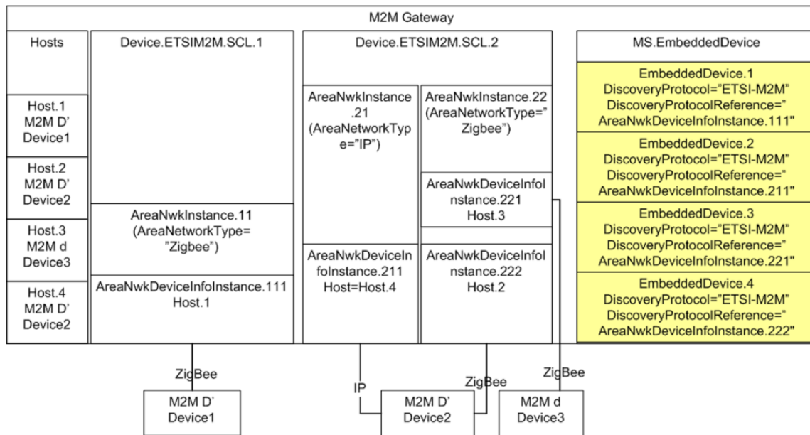
Figure 51: M2M Device Discovery for Proxy Management
