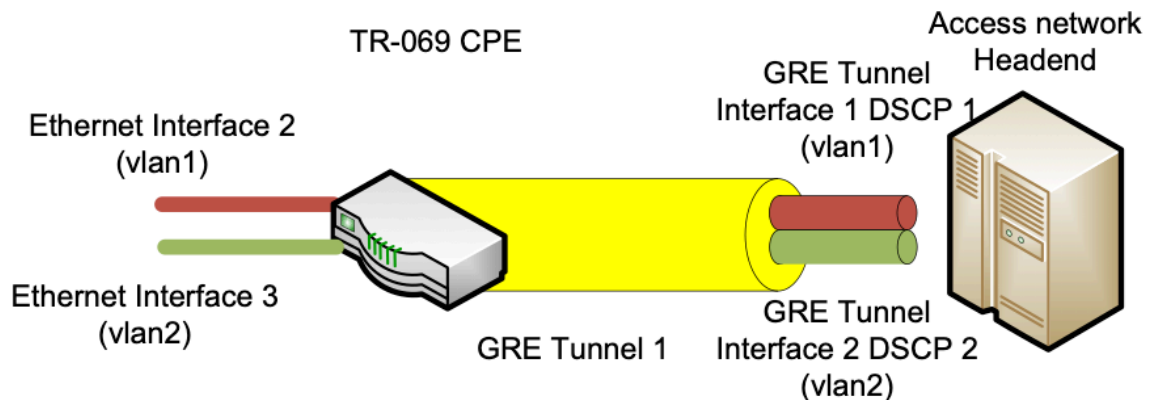
Figure 59: VLAN Traffic over GRE
