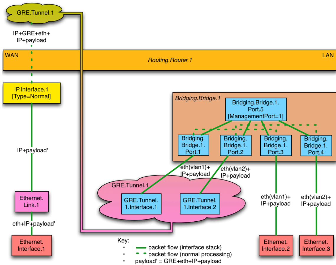
Figure 60: L2 over GRE Tunnel
