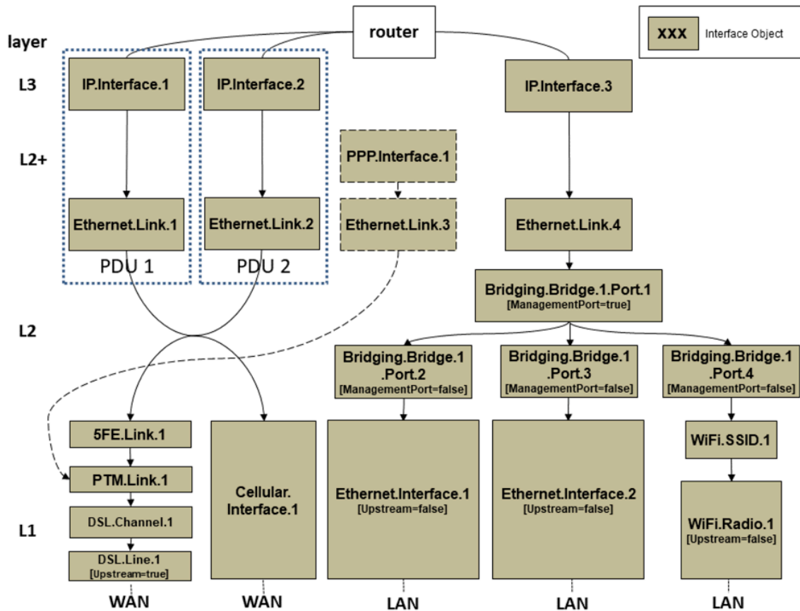
Figure 82: Hybrid access example
