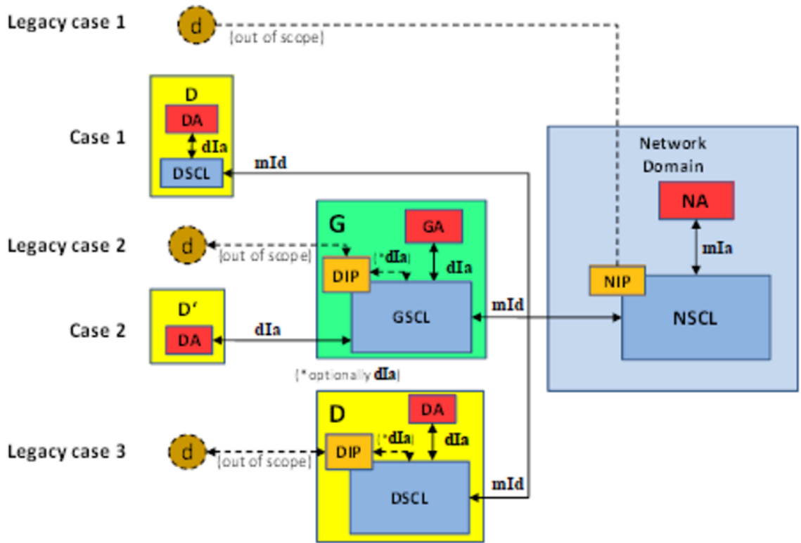
Figure 49: ETSI M2M Devices and Gateways
