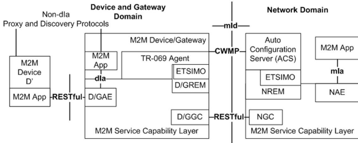
Figure 48: M2M REM Service Capability
