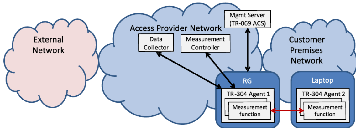
Figure 71: TR-304 Framework
