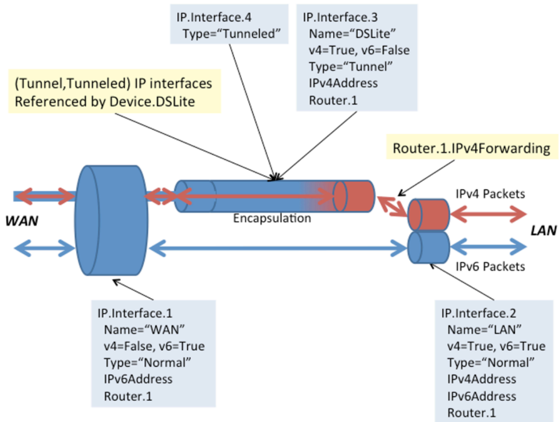
Figure 40: Sample DS-Lite Routing and Forwarding
