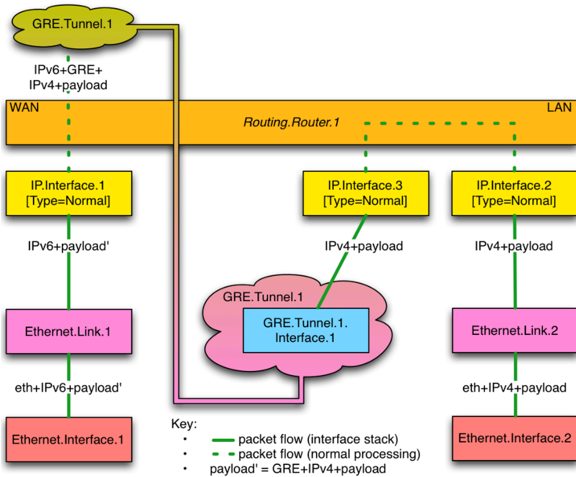
Figure 62: L3 over GRE Tunnel
