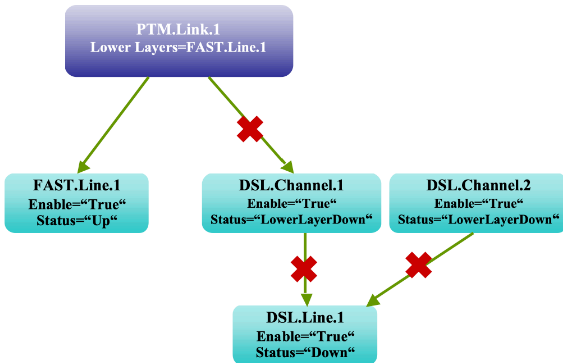
Figure 67: PTM Link for FAST mode Line
