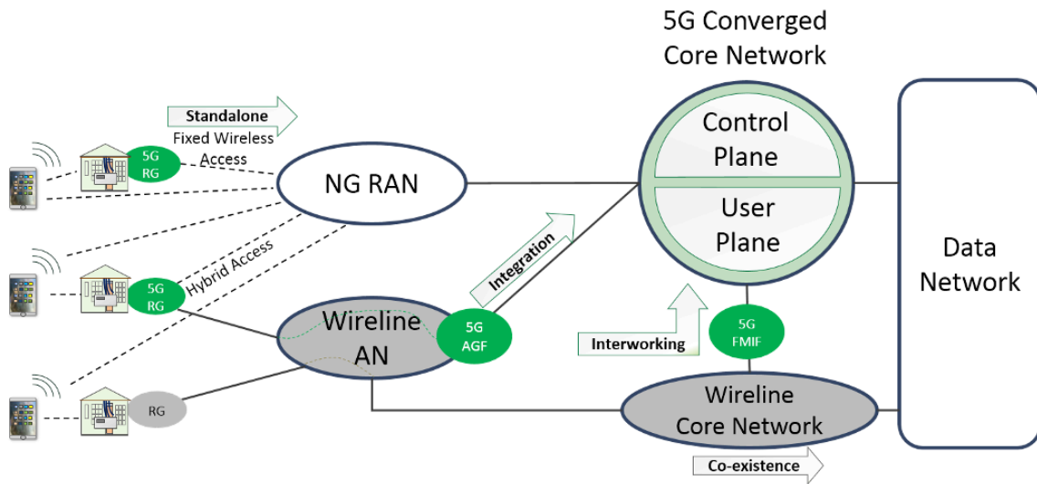
Figure 78: 5G Converged Core Network
