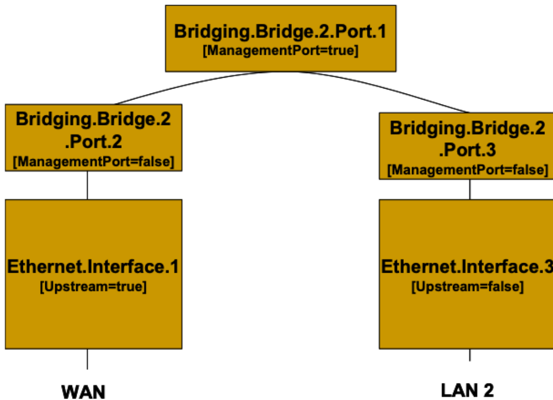
Figure 27: Bridge 2 model
