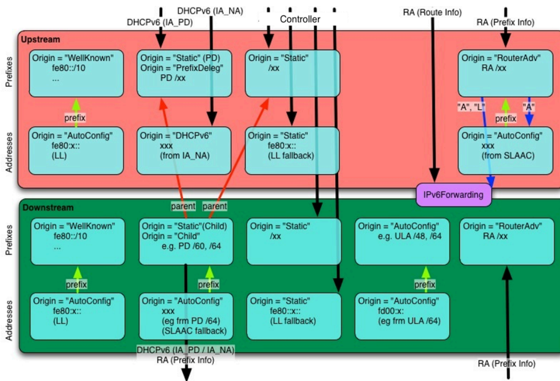
Figure 37: Internal Relationships of IPv6 Addresses and Prefixes
