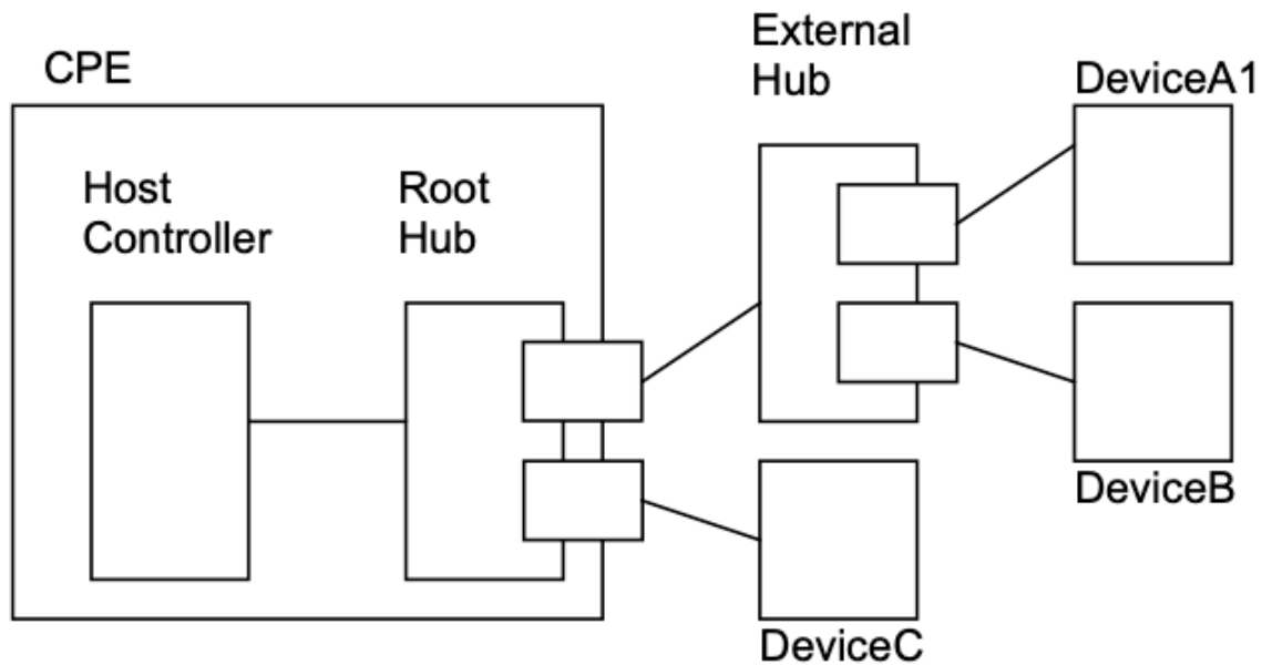
Figure 70: Example USB Host Connections
