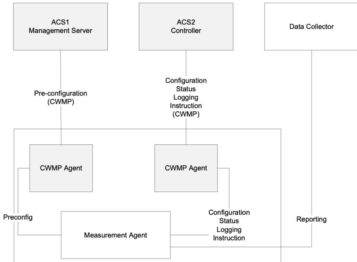
Figure 76: CWMP Multi-ACS Deployment
