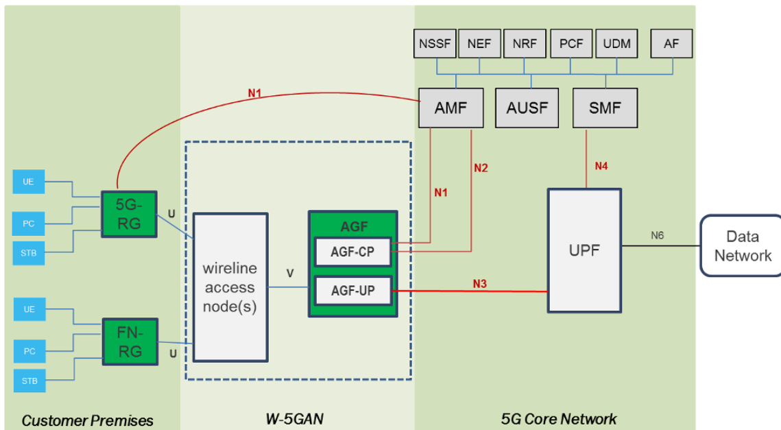
Figure 79: 5G Architecture
