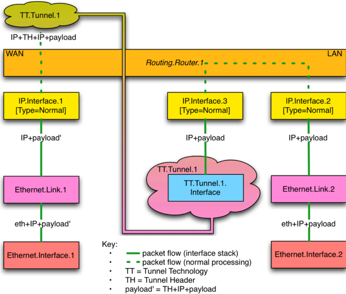
Figure 20: General Layer 3 Tunneling Interface Stack
