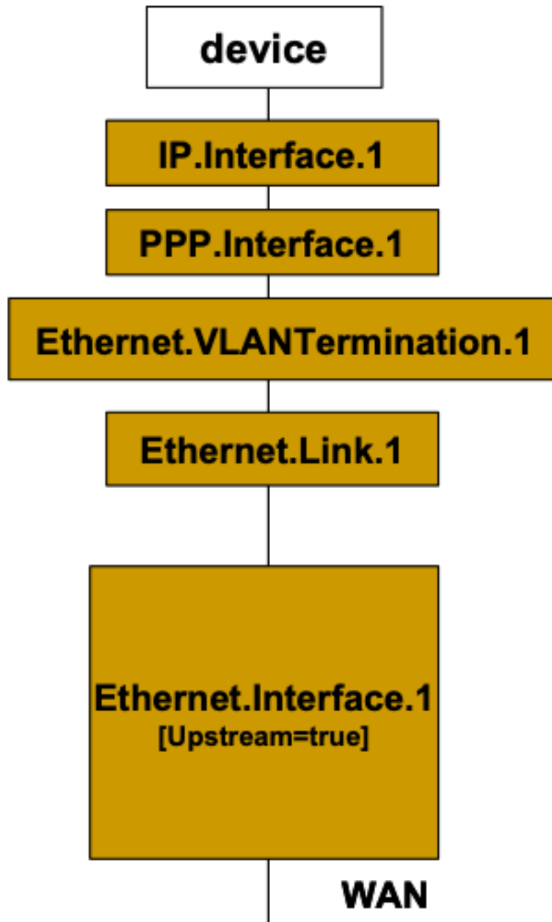
Figure 29: VLAN Termination model
