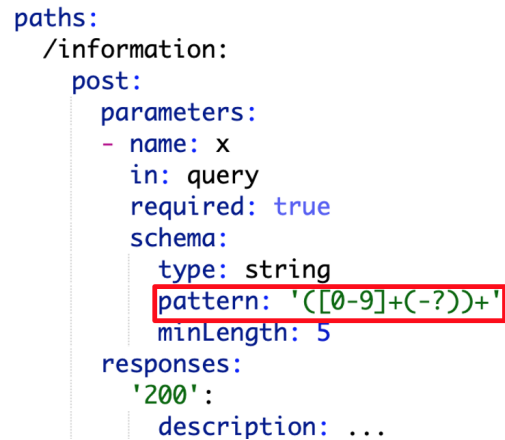
(b) Sanitization in OpenAPI-based web API. Regexes are supported to encode string constraints in popular web API schema definition languages including OpenAPI [9], RAML [5], and API Blueprint [1].
