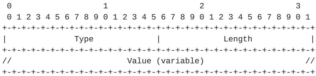
Figure 4: TLV Format
