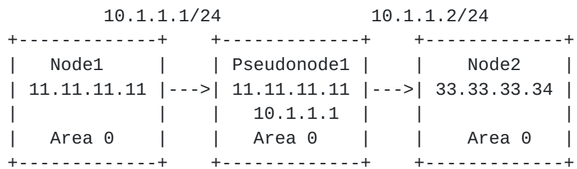
Figure 33: OSPF Pseudonodes
