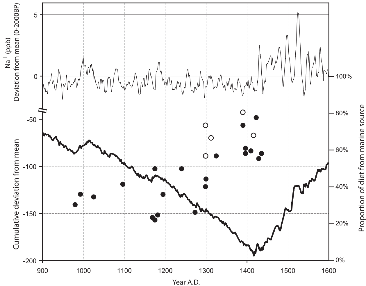
Figure 6. The Na + concentration (sea salt) time series, a proxy record of storminess, from GISP2, shown against human isotopic data —lower RHS scale showing proportion of diet from marine sources (Arneborg et al. 1999; Meeker and Mayewski 2002; data from Greenland Ice Sheet Project 2. http://www.gisp2.sr.unh.edu/ ): The Na + in the Greenland icecap derives principally from sea salt in the North Atlantic (Meeker and Mayewski 2002), so temporal variations in sea salt concentrations in the GISP2 record represent a proxy record for winter storminess in the North Atlantic. The upper line (top LHS scale) is the 5 year running mean of deviations from the long term mean. The lower line (RHS scale) is the same data presented as cumulative deviations (see text for explanation). Storminess is an indicator of regional circulation change in the North Atlantic, and perhaps unsurprisingly this regional measure of change does not show a strong correlation with evidence of dietary changes in Greenland but the most significant shift occurs within a short time of the final extinction of the Norse settlement. Closed circles data from the Eastern Settlement, open circles data from the Western Settlement.
