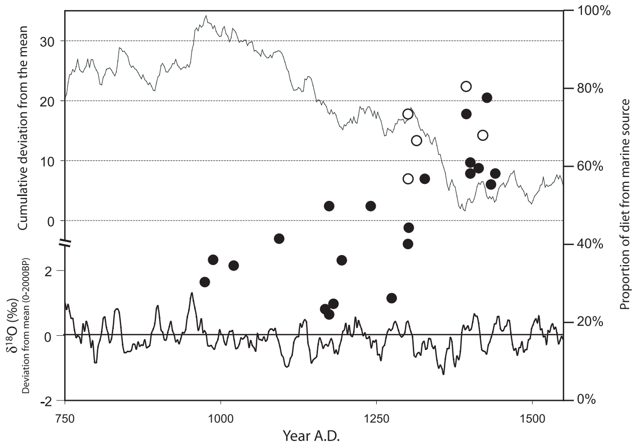
Figure 5. The \delta^{18}\text{O} time series from GISP2 (LHS scale), a proxy temperature record, shown against human isotopic data (RHS scale showing proportion of diet from marine sources) (Arneborg et al. 1999; Mayewski et al. 1993; Mayewski and White 2002; data from Greenland Ice Sheet Project 2. http://www.gisp2.sr.unh.edu/ ): Comparisons of \delta^{18}\text{O} time series for GISP2 and meteorological records for West Greenland for the period 1860 A.D. to the present demonstrate a statistical relationship between the \delta^{18}\text{O} time series and mean winter air temperatures across West Greenland (Barlow 2001; Dawson et al. 2003). The lower line is the 5 year running mean of deviations from the long term mean. The upper line is the same data presented as cumulative deviations (see text for explanation). The points represent isotopic data on Norse Greenlanders showing the proportion of marine food consumed. The change in the cumulative deviation — marking a shift to cooler condition — also marks the time of a distinct shift in the isotopic records of diet. Closed circles data from the Eastern Settlement, open circles data from the Western Settlement.
