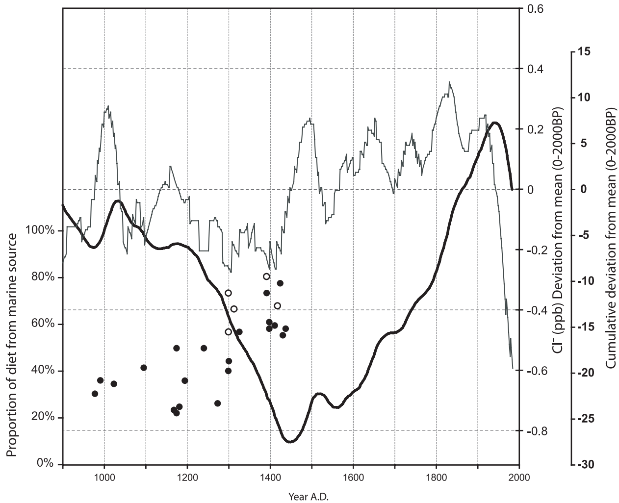
Figure 7. The proxy record of sea ice from GISP2 –RHS scales, bold figures cumulative scale (Dugmore et al. in press; Mayewski et al. 1993) shown against human isotopic data, RHS scale showing proportion of diet from marine sources (Arneborg et al. 1999): The upper line is the 5 year running mean of deviations from the long term mean (data from Greenland Ice Sheet Project 2. http://www.gisp2.sr.unh.edu/ ). The lower line is the same data presented as cumulative deviations (see text for explanation). The most significant shift of the cumulative measure (most pronounced change in over 400 years, when past experience of anticyclonic conditions/sea ice extent were becoming the poorest indicator of future trajectories of change) occurs within a short time of the final extinction of the Norse settlement. Closed circles data from the Eastern Settlement, open circles data from the Western Settlement.
