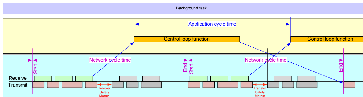
513 514 Figure 18 – network cycle and non-isochronous application (Basic model)
