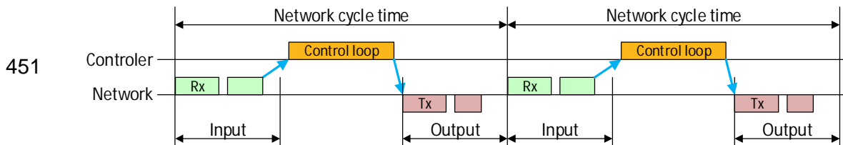
451 Figure 13 – Variation 4: one cycle timing model
