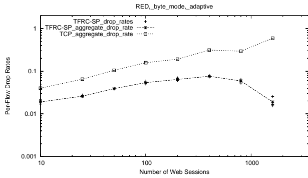
Figure 20: Drop and Send Rates with Adaptive RED Queues in Byte Mode
