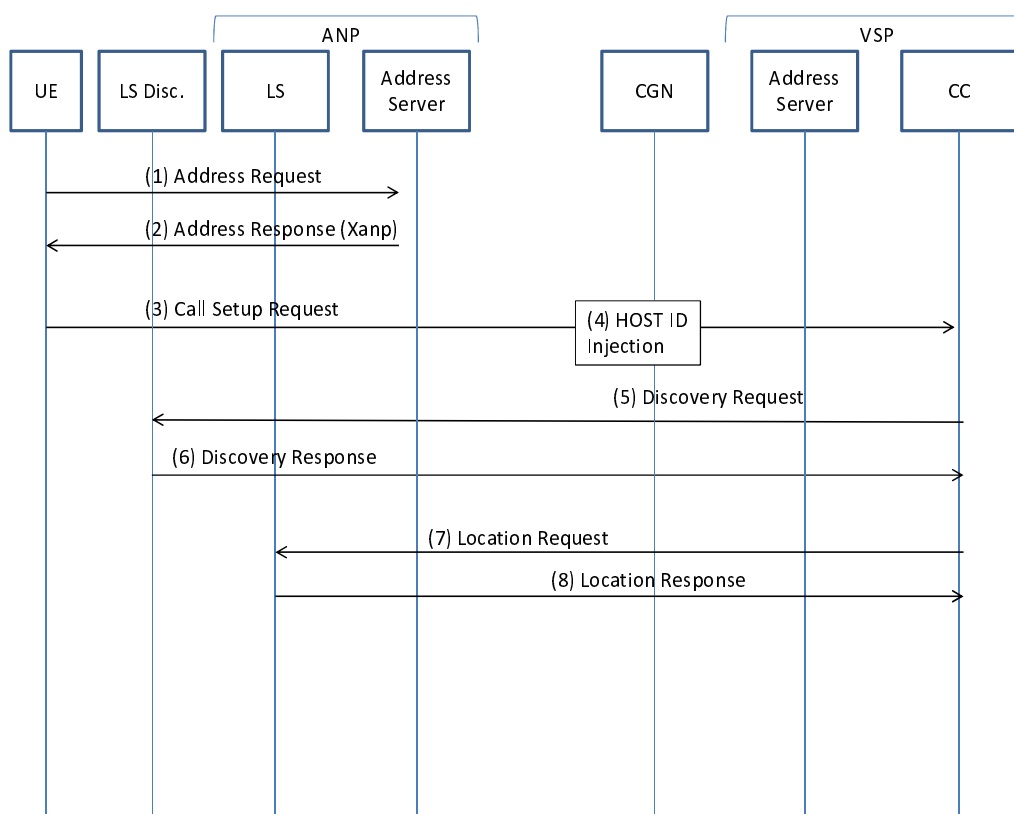
Figure A.5: Location retrieval with a CGN
