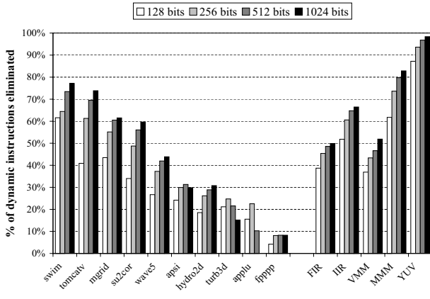
Figure 8: Percentage of dynamic instructions eliminated by SLP analysis for a variety of hypothetical datapath widths.
