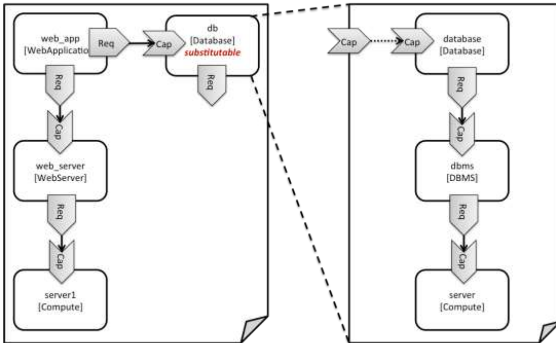
441 Figure 1: Using template substitution to implement a database tier
